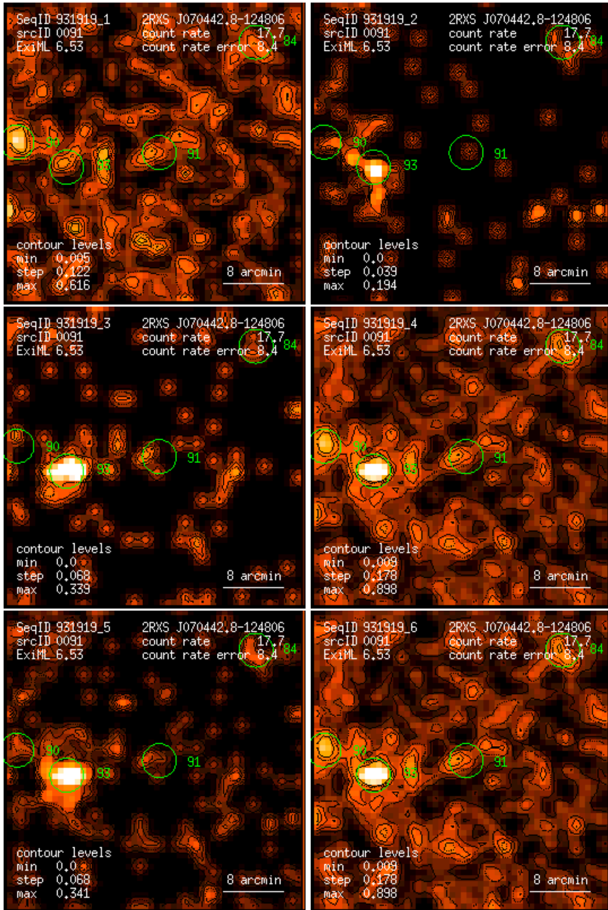
Figure 91: RASS 931919: detection 0091: band rate images, Gaussian filter: (1) PSPC channels 11 – 41, (2) 52 – 90, (3) 91 – 201, (4) 11 – 235, (5) 52 – 201, (6) 11 – 201. Broad band rates in counts/ks. Band rate contour levels in counts/ks/arcmin 2 .
