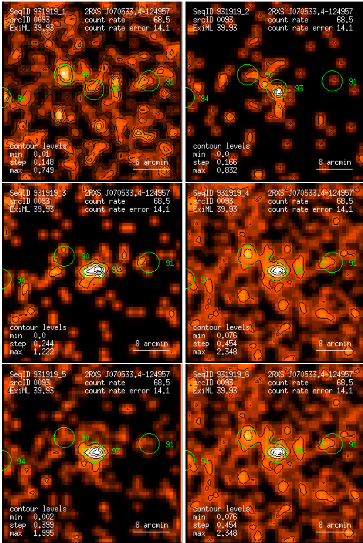
Figure 93: RASS 931919: detection 0093: band rate images, Gaussian filter: (1) PSPC channels 11 – 41, (2) 52 – 90, (3) 91 – 201, (4) 11 – 235, (5) 52 – 201, (6) 11 – 201. Broad band rates in counts/ks. Band rate contour levels in counts/ks/arcmin 2 .
