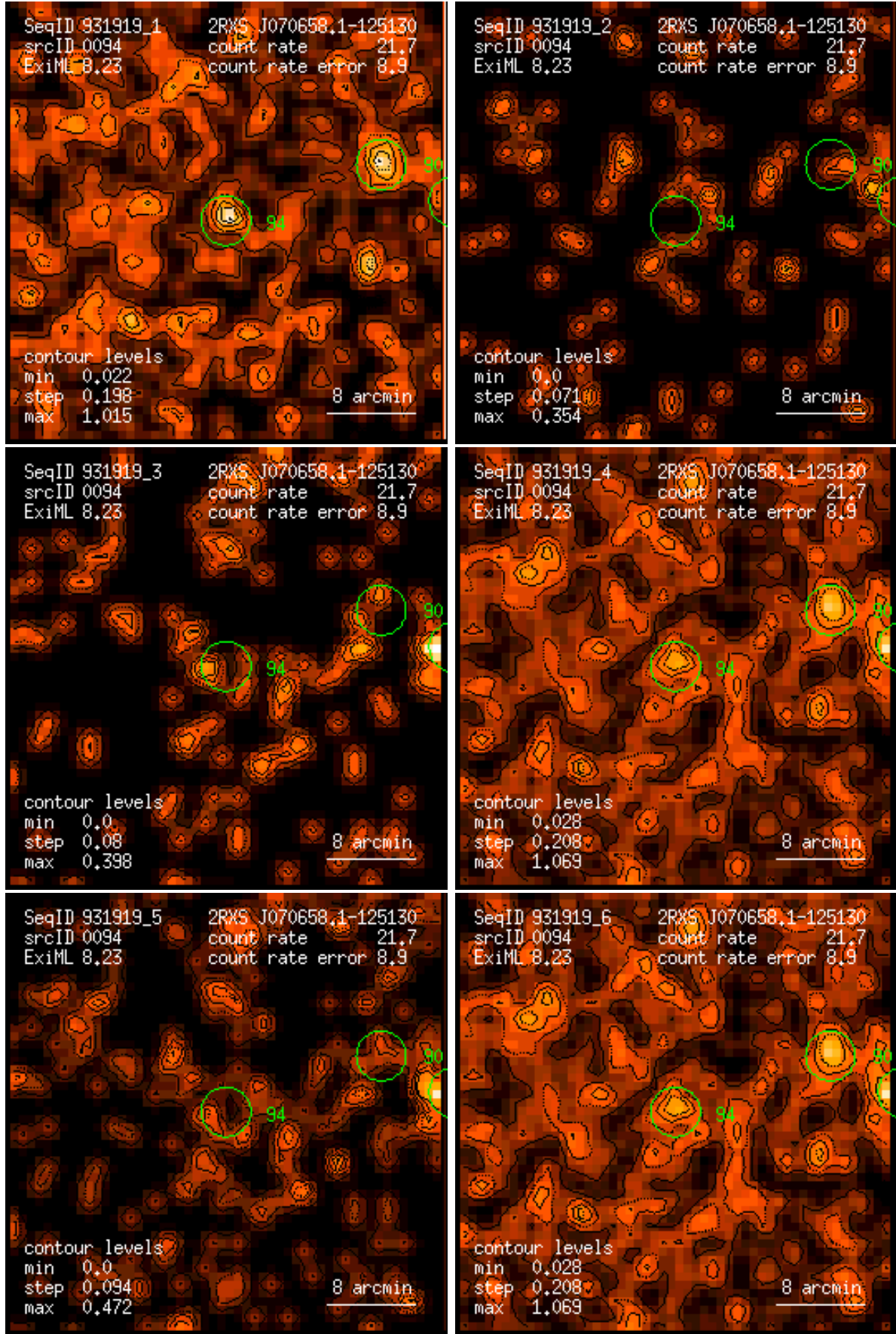
Figure 94: RASS 931919: detection 0094: band rate images, Gaussian filter: (1) PSPC channels 11 – 41, (2) 52 – 90, (3) 91 – 201, (4) 11 – 235, (5) 52 – 201, (6) 11 – 201. Broad band rates in counts/ks. Band rate contour levels in counts/ks/arcmin 2 .
