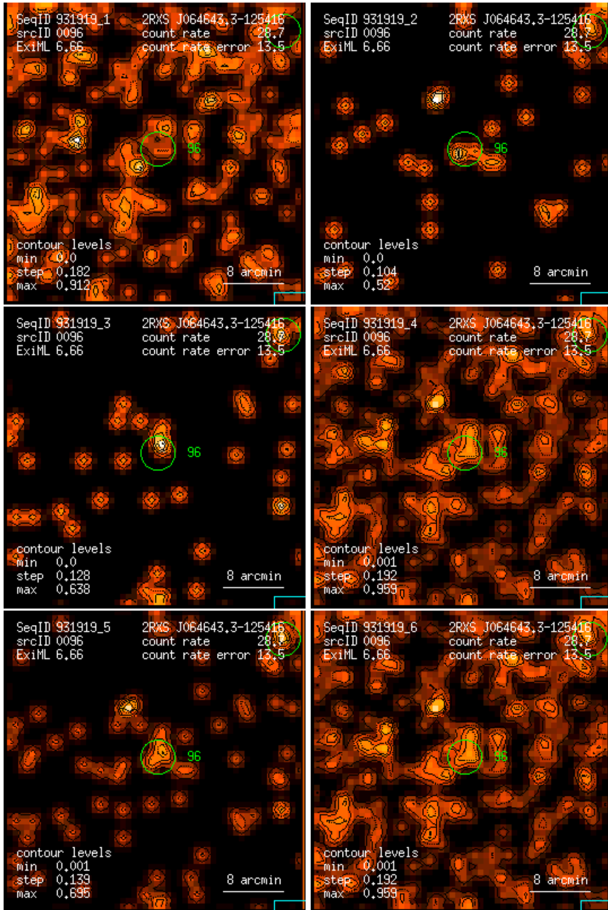
Figure 96: RASS 931919: detection 0096: band rate images, Gaussian filter: (1) PSPC channels 11 – 41, (2) 52 – 90, (3) 91 – 201, (4) 11 – 235, (5) 52 – 201, (6) 11 – 201. Broad band rates in counts/ks. Band rate contour levels in counts/ks/arcmin 2 .
