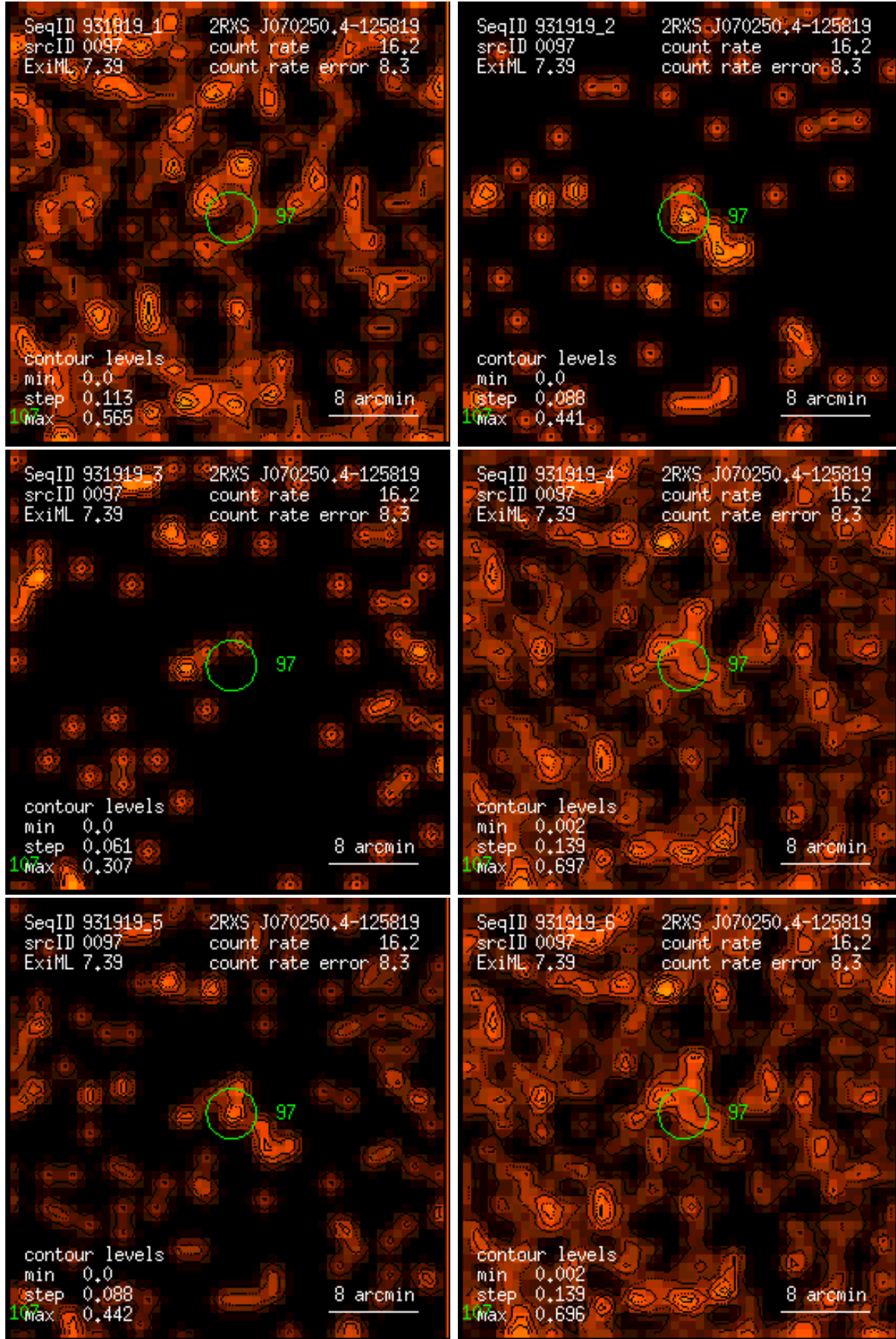
Figure 97: RASS 931919: detection 0097: band rate images, Gaussian filter: (1) PSPC channels 11 – 41, (2) 52 – 90, (3) 91 – 201, (4) 11 – 235, (5) 52 – 201, (6) 11 – 201. Broad band rates in counts/ks. Band rate contour levels in counts/ks/arcmin 2 .
