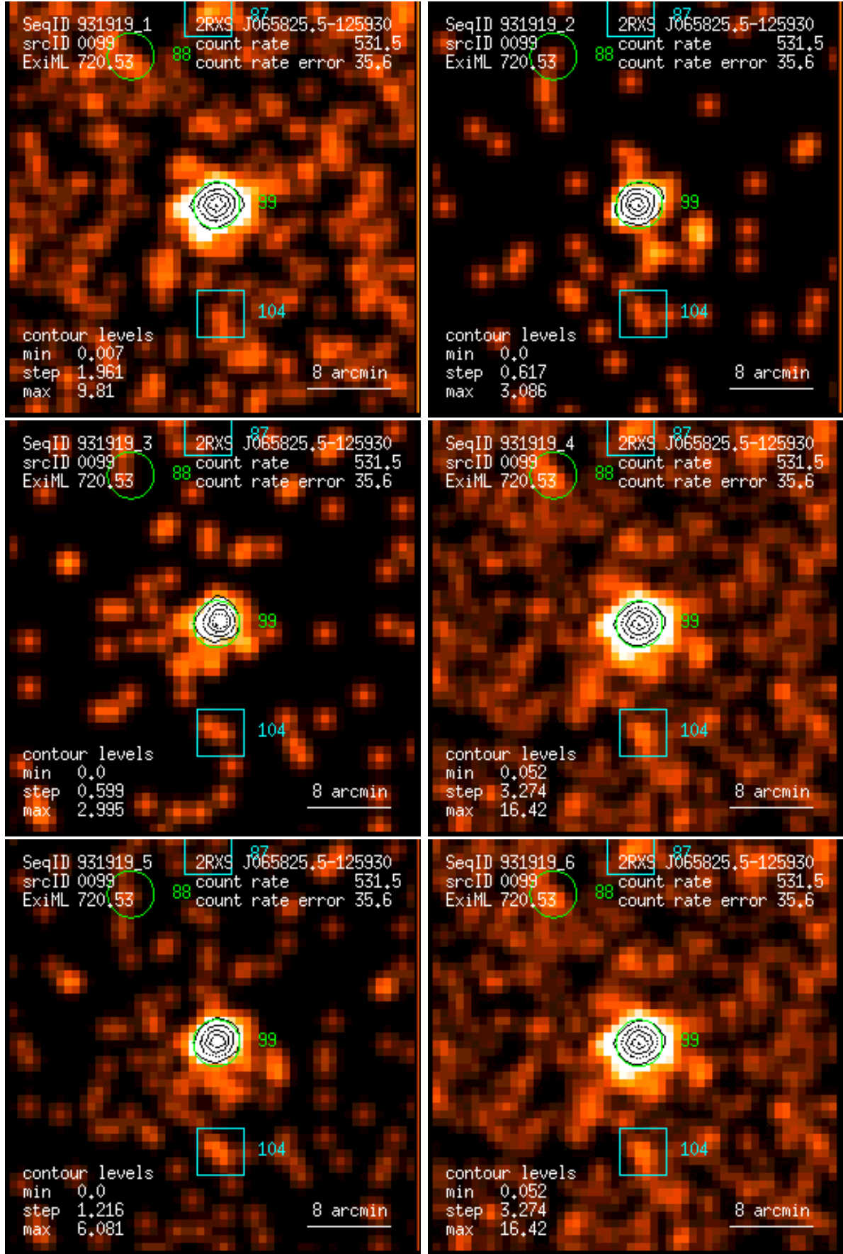
Figure 99: RASS 931919: detection 0099: band rate images, Gaussian filter: (1) PSPC channels 11 – 41, (2) 52 – 90, (3) 91 – 201, (4) 11 – 235, (5) 52 – 201, (6) 11 – 201. Broad band rates in counts/ks. Band rate contour levels in counts/ks/arcmin 2 .
