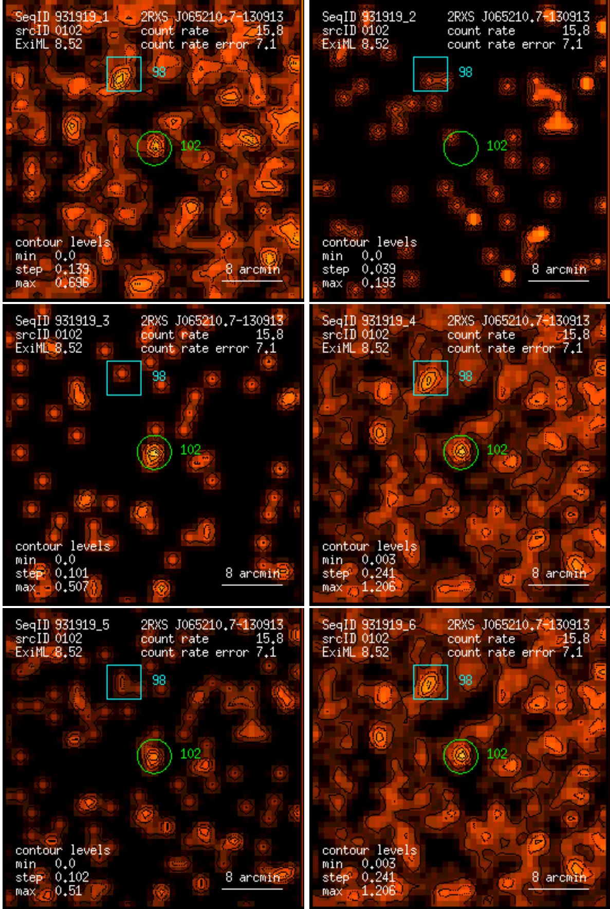
Figure 102: RASS 931919: detection 0102: band rate images, Gaussian filter: (1) PSPC channels 11 – 41, (2) 52 – 90, (3) 91 – 201, (4) 11 – 235, (5) 52 – 201, (6) 11 – 201. Broad band rates in counts/ks. Band rate contour levels in counts/ks/arcmin 2 .
