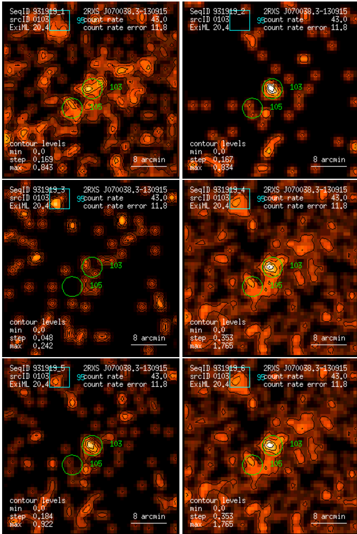
Figure 103: RASS 931919: detection 0103: band rate images, Gaussian filter: (1) PSPC channels 11 – 41, (2) 52 – 90, (3) 91 – 201, (4) 11 – 235, (5) 52 – 201, (6) 11 – 201. Broad band rates in counts/ks. Band rate contour levels in counts/ks/arcmin 2 .
