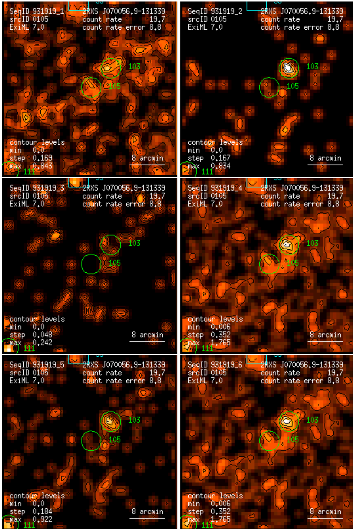
Figure 105: RASS 931919: detection 0105: band rate images, Gaussian filter: (1) PSPC channels 11 – 41, (2) 52 – 90, (3) 91 – 201, (4) 11 – 235, (5) 52 – 201, (6) 11 – 201. Broad band rates in counts/ks. Band rate contour levels in counts/ks/arcmin 2 .
