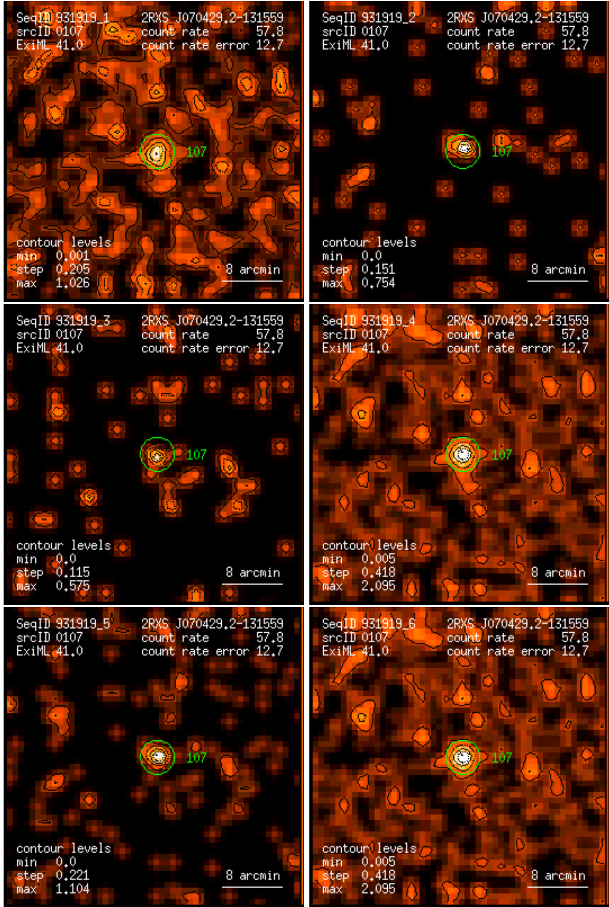
Figure 107: RASS 931919: detection 0107: band rate images, Gaussian filter: (1) PSPC channels 11 – 41, (2) 52 – 90, (3) 91 – 201, (4) 11 – 235, (5) 52 – 201, (6) 11 – 201. Broad band rates in counts/ks. Band rate contour levels in counts/ks/arcmin 2 .
