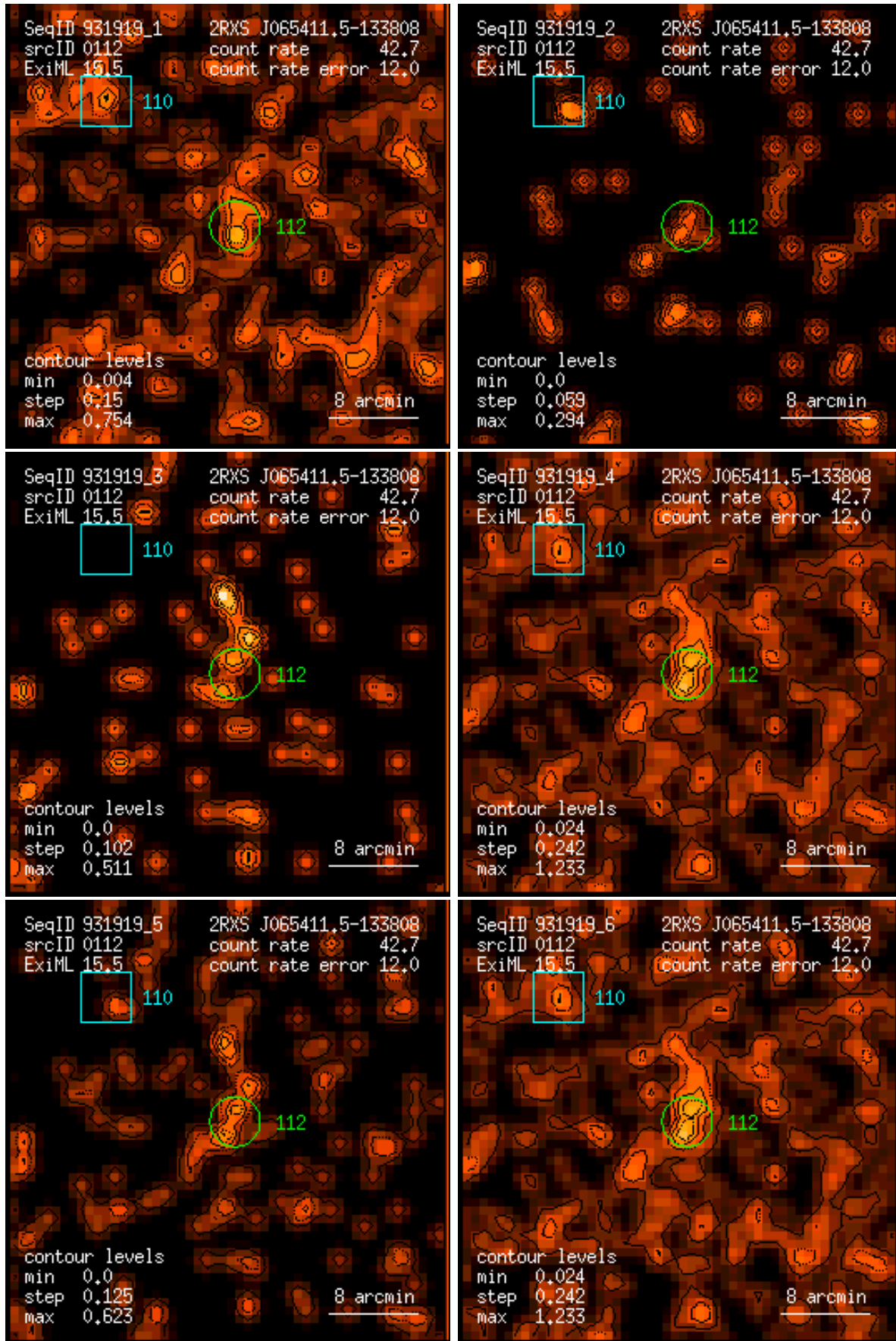
Figure 112: RASS 931919: detection 0112: band rate images, Gaussian filter: (1) PSPC channels 11 – 41, (2) 52 – 90, (3) 91 – 201, (4) 11 – 235, (5) 52 – 201, (6) 11 – 201. Broad band rates in counts/ks. Band rate contour levels in counts/ks/arcmin 2 .
