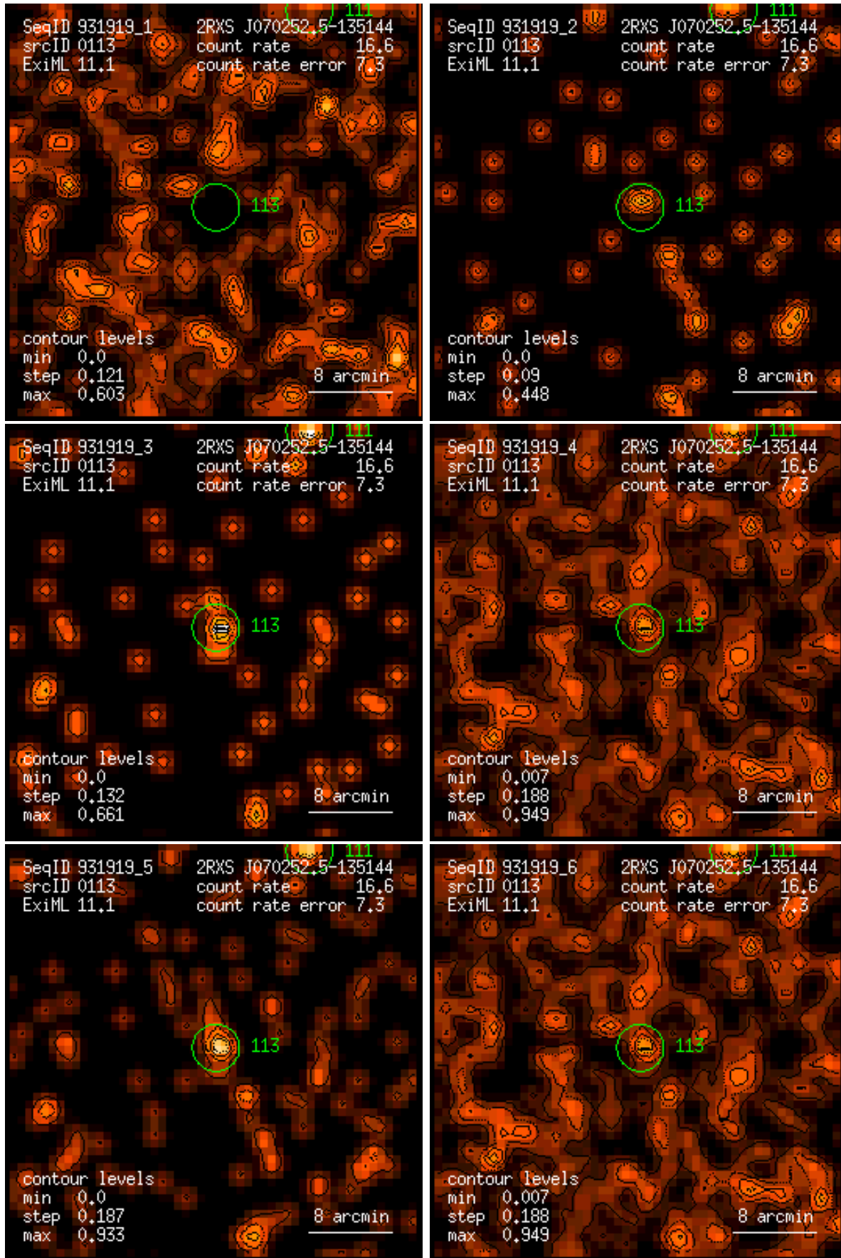
Figure 113: RASS 931919: detection 0113: band rate images, Gaussian filter: (1) PSPC channels 11 – 41, (2) 52 – 90, (3) 91 – 201, (4) 11 – 235, (5) 52 – 201, (6) 11 – 201. Broad band rates in counts/ks. Band rate contour levels in counts/ks/arcmin 2 .
