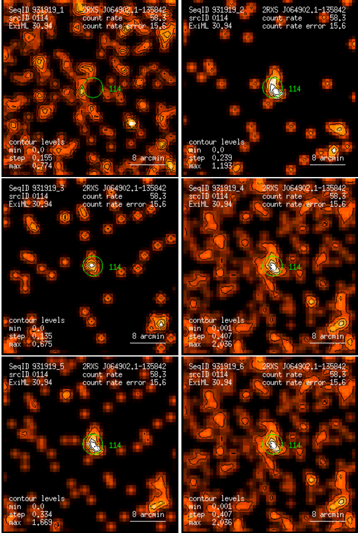
Figure 114: RASS 931919: detection 0114: band rate images, Gaussian filter: (1) PSPC channels 11 – 41, (2) 52 – 90, (3) 91 – 201, (4) 11 – 235, (5) 52 – 201, (6) 11 – 201. Broad band rates in counts/ks. Band rate contour levels in counts/ks/arcmin 2 .
