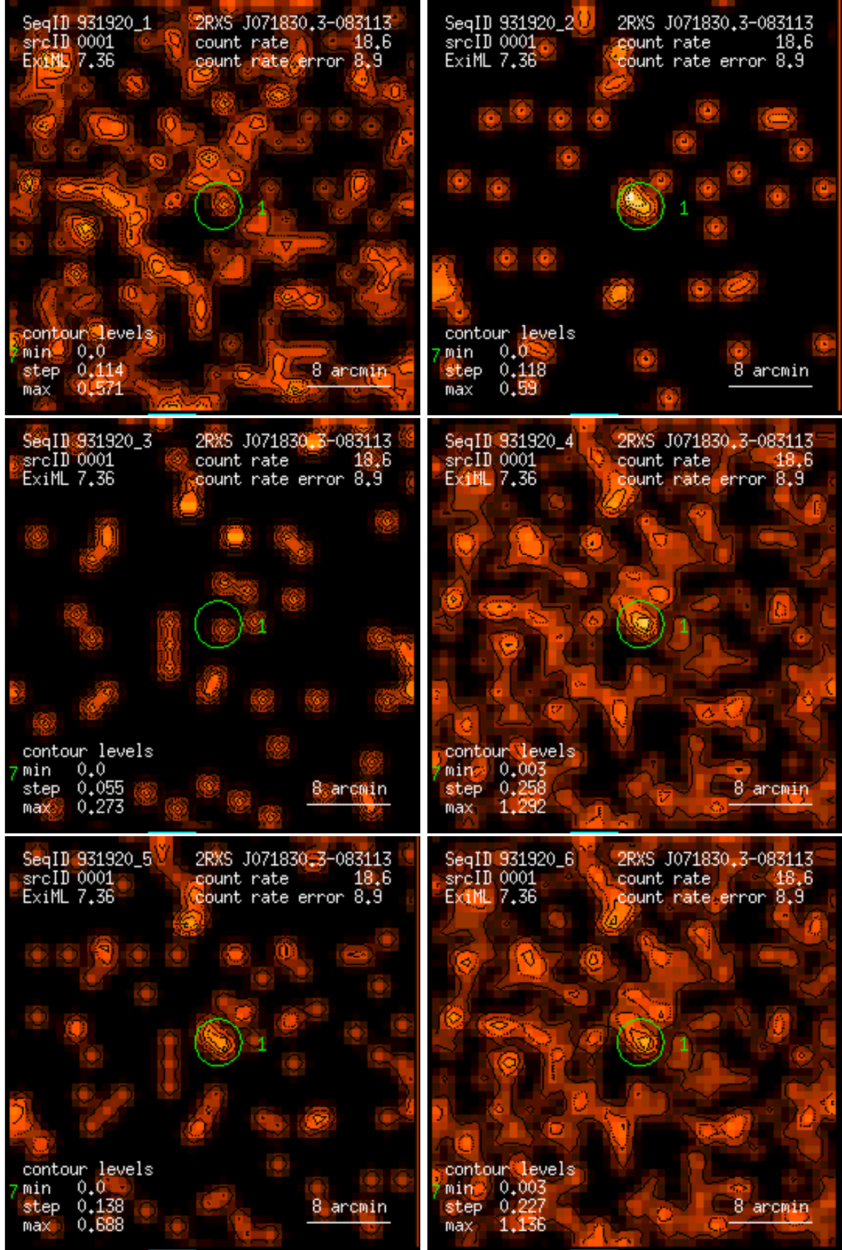
Figure 1: RASS 931920: detection 0001: band rate images, Gaussian filter: (1) PSPC channels 11 – 41, (2) 52 – 90, (3) 91 – 201, (4) 11 – 235, (5) 52 – 201, (6) 11 – 201. Broad band rates in counts/ks. Band rate contour levels in counts/ks/arcmin 2 .
