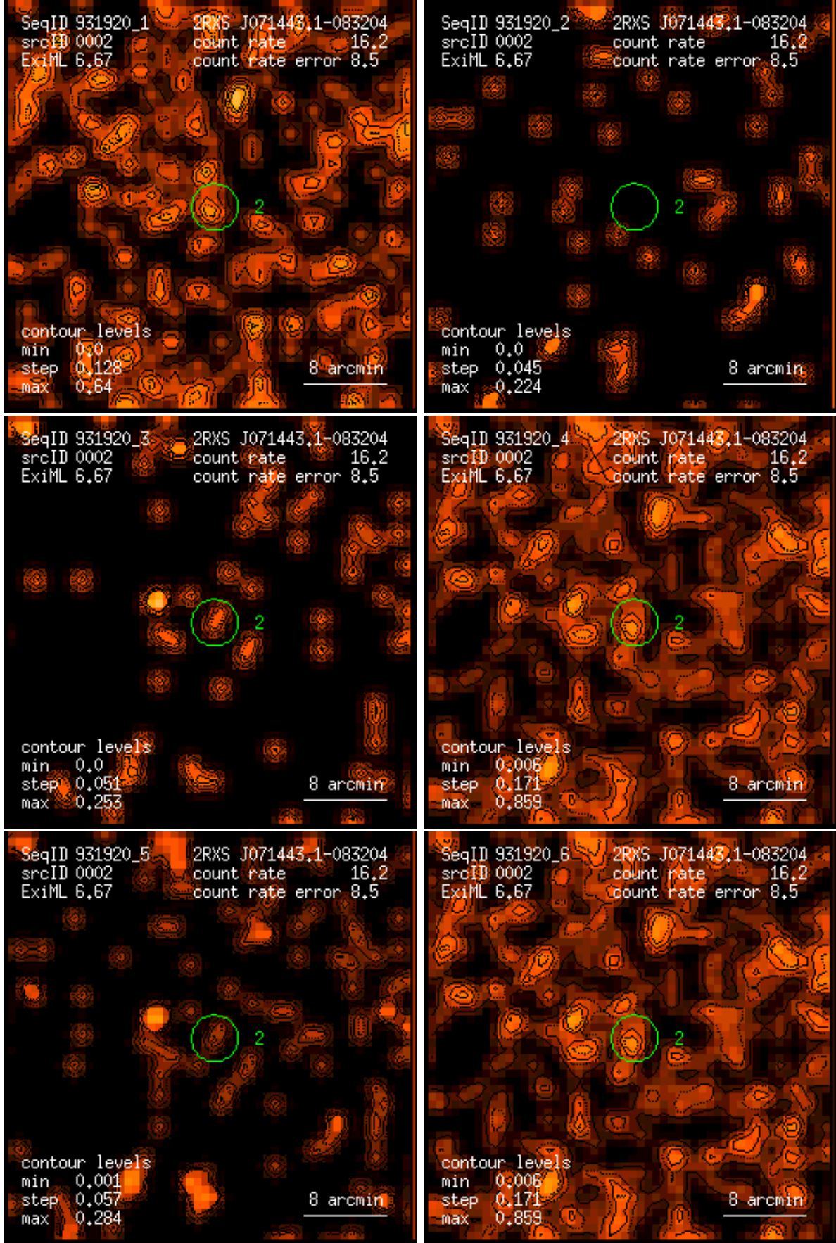
Figure 2: RASS 931920: detection 0002: band rate images, Gaussian filter: (1) PSPC channels 11 – 41, (2) 52 – 90, (3) 91 – 201, (4) 11 – 235, (5) 52 – 201, (6) 11 – 201. Broad band rates in counts/ks. Band rate contour levels in counts/ks/arcmin 2 .
