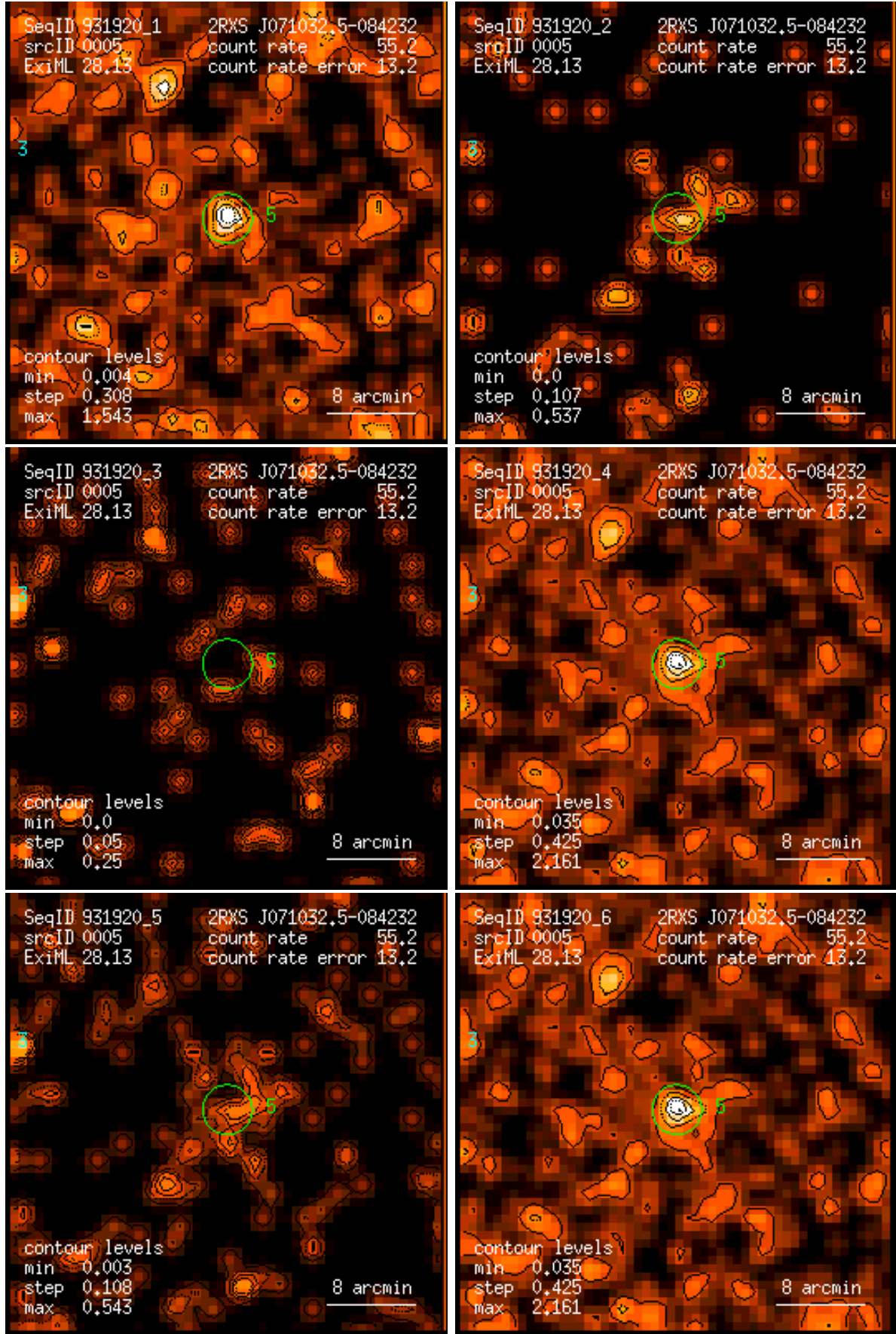
Figure 5: RASS 931920: detection 0005: band rate images, Gaussian filter: (1) PSPC channels 11 – 41, (2) 52 – 90, (3) 91 – 201, (4) 11 – 235, (5) 52 – 201, (6) 11 – 201. Broad band rates in counts/ks. Band rate contour levels in counts/ks/arcmin 2 .
