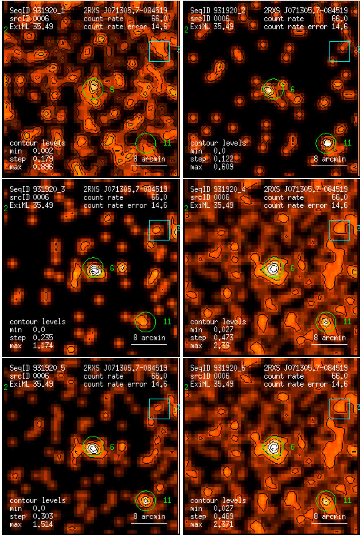
Figure 6: RASS 931920: detection 0006: band rate images, Gaussian filter: (1) PSPC channels 11 – 41, (2) 52 – 90, (3) 91 – 201, (4) 11 – 235, (5) 52 – 201, (6) 11 – 201. Broad band rates in counts/ks. Band rate contour levels in counts/ks/arcmin 2 .
