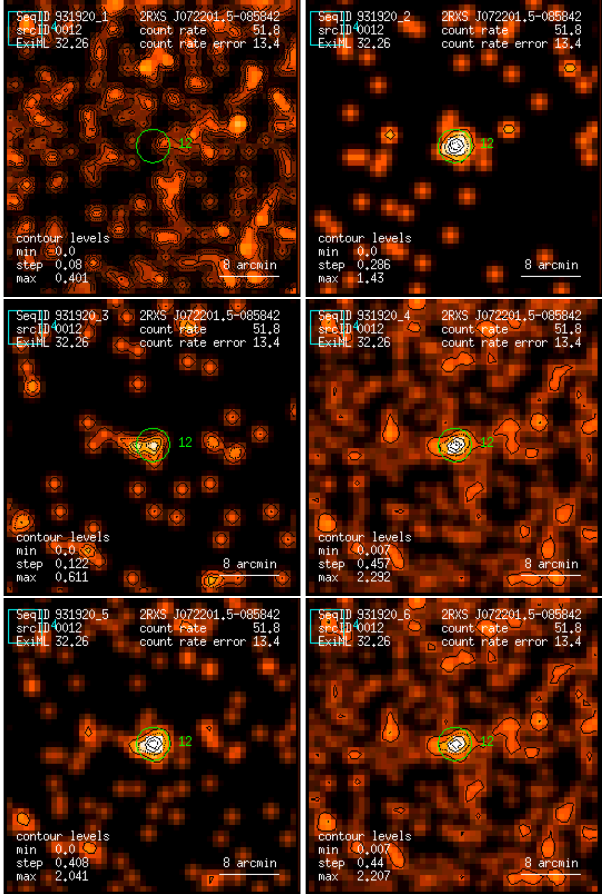
Figure 12: RASS 931920: detection 0012: band rate images, Gaussian filter: (1) PSPC channels 11 – 41, (2) 52 – 90, (3) 91 – 201, (4) 11 – 235, (5) 52 – 201, (6) 11 – 201. Broad band rates in counts/ks. Band rate contour levels in counts/ks/arcmin 2 .
