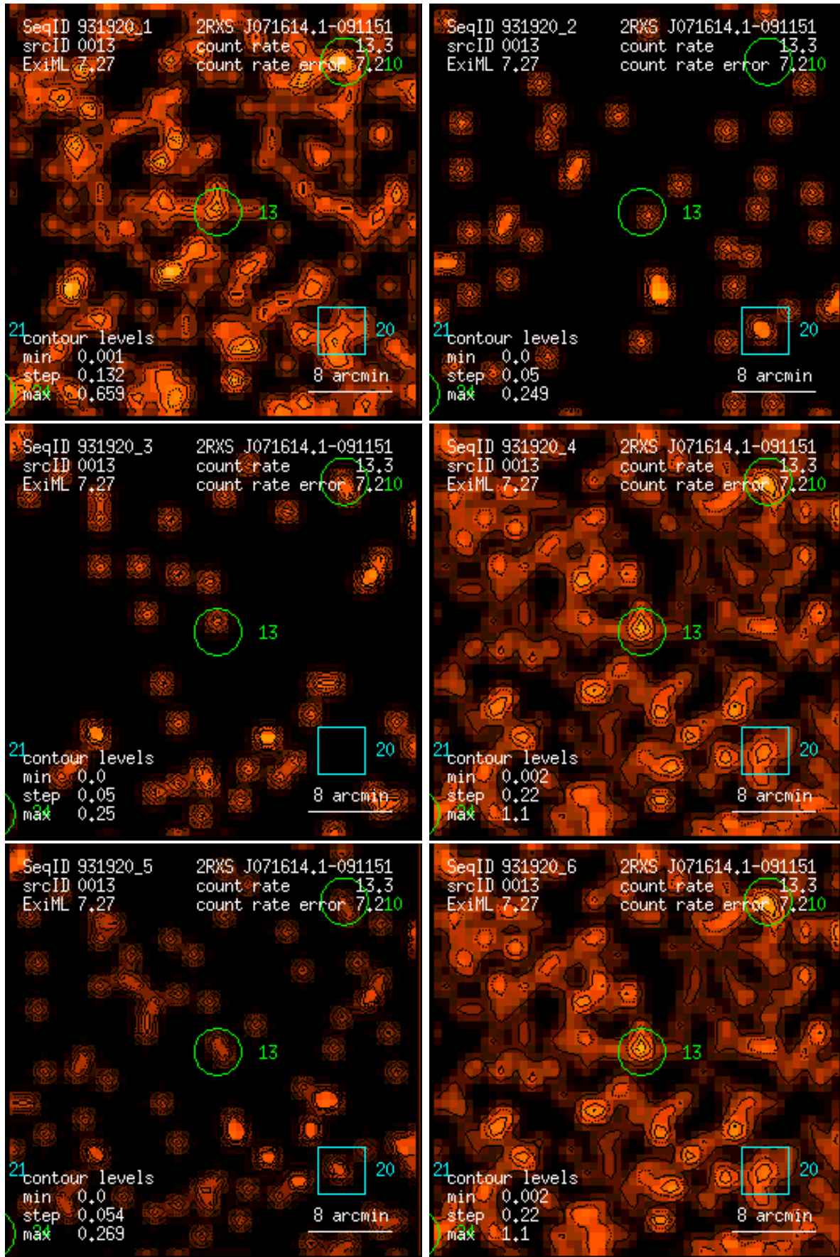
Figure 13: RASS 931920: detection 0013: band rate images, Gaussian filter: (1) PSPC channels 11 – 41, (2) 52 – 90, (3) 91 – 201, (4) 11 – 235, (5) 52 – 201, (6) 11 – 201. Broad band rates in counts/ks. Band rate contour levels in counts/ks/arcmin 2 .
