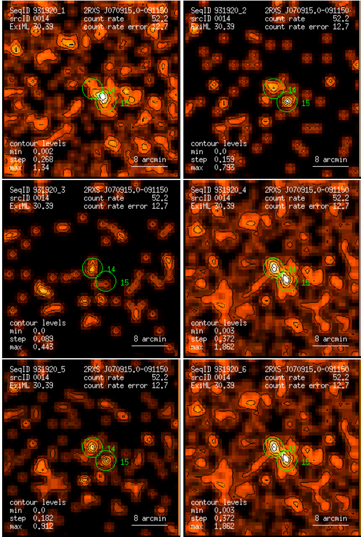
Figure 14: RASS 931920: detection 0014: band rate images, Gaussian filter: (1) PSPC channels 11 – 41, (2) 52 – 90, (3) 91 – 201, (4) 11 – 235, (5) 52 – 201, (6) 11 – 201. Broad band rates in counts/ks. Band rate contour levels in counts/ks/arcmin 2 .
