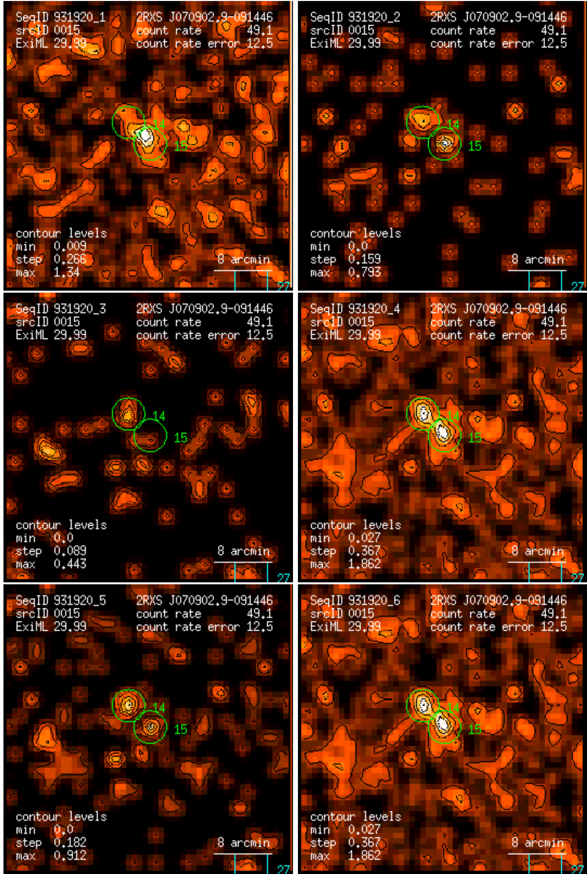
Figure 15: RASS 931920: detection 0015: band rate images, Gaussian filter: (1) PSPC channels 11 – 41, (2) 52 – 90, (3) 91 – 201, (4) 11 – 235, (5) 52 – 201, (6) 11 – 201. Broad band rates in counts/ks. Band rate contour levels in counts/ks/arcmin 2 .
