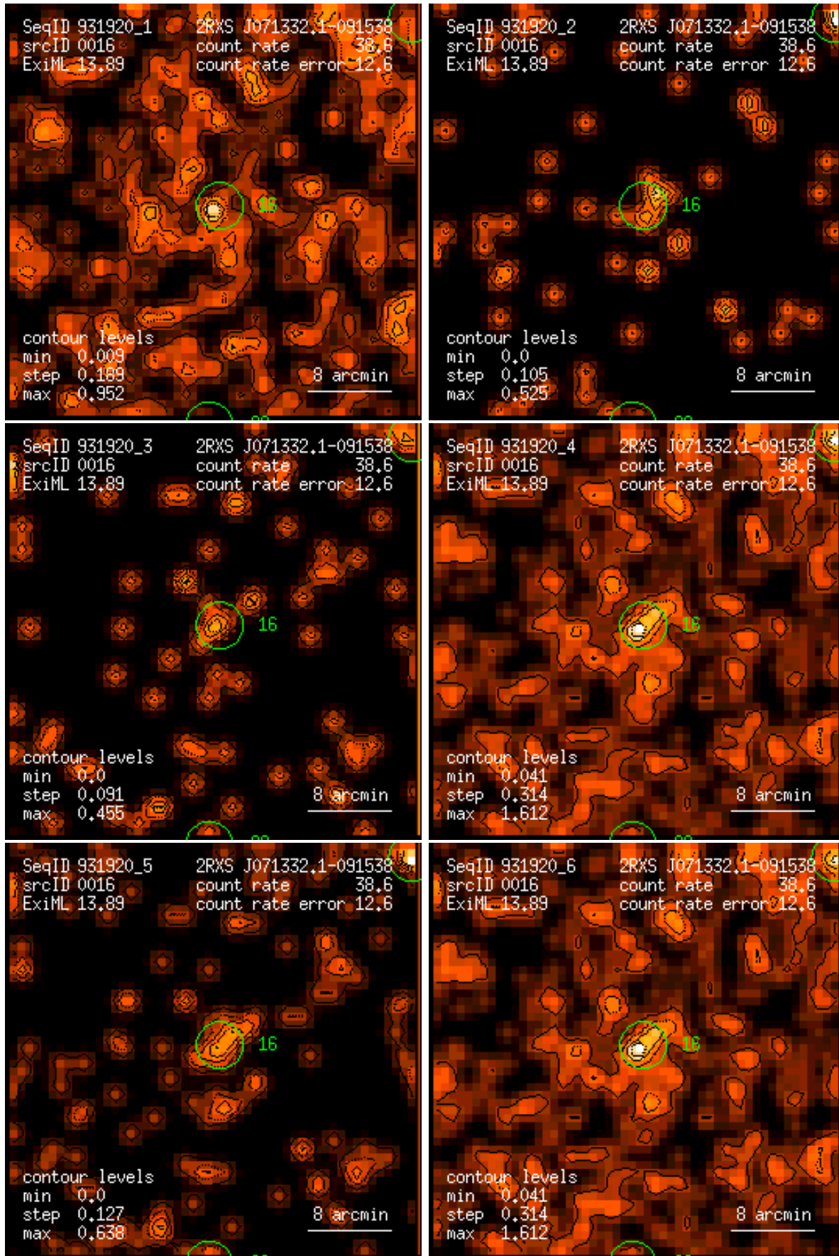
Figure 16: RASS 931920: detection 0016: band rate images, Gaussian filter: (1) PSPC channels 11 – 41, (2) 52 – 90, (3) 91 – 201, (4) 11 – 235, (5) 52 – 201, (6) 11 – 201. Broad band rates in counts/ks. Band rate contour levels in counts/ks/arcmin 2 .
