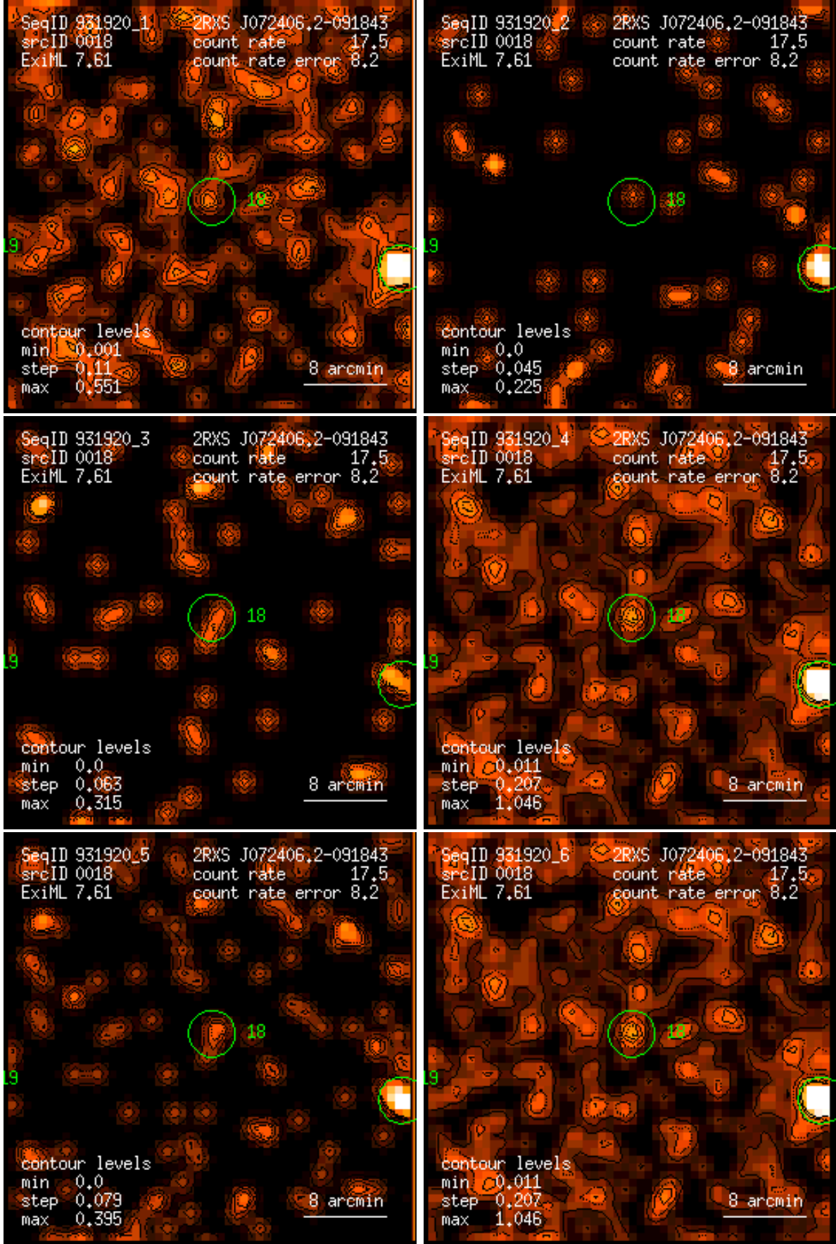
Figure 18: RASS 931920: detection 0018: band rate images, Gaussian filter: (1) PSPC channels 11 – 41, (2) 52 – 90, (3) 91 – 201, (4) 11 – 235, (5) 52 – 201, (6) 11 – 201. Broad band rates in counts/ks. Band rate contour levels in counts/ks/arcmin 2 .
