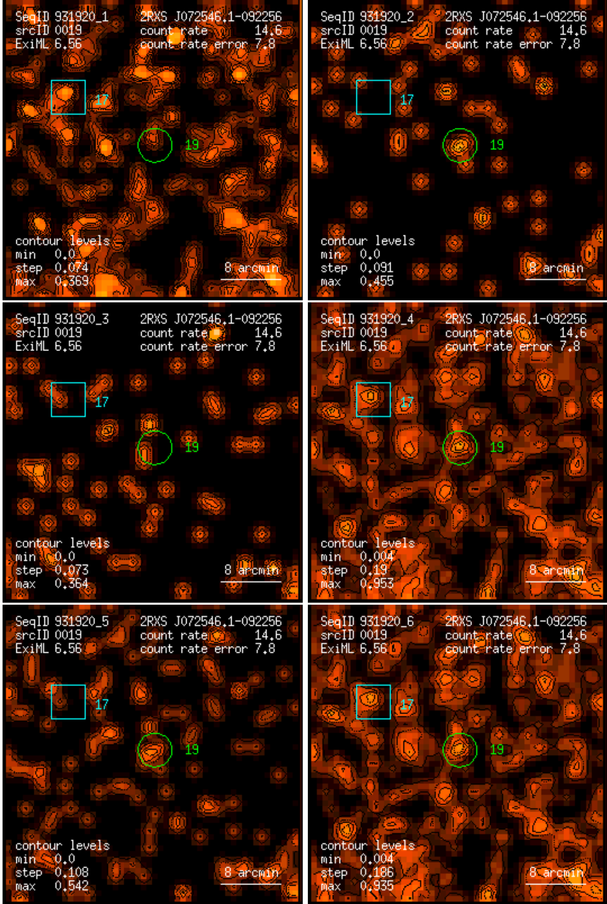
Figure 19: RASS 931920: detection 0019: band rate images, Gaussian filter: (1) PSPC channels 11 – 41, (2) 52 – 90, (3) 91 – 201, (4) 11 – 235, (5) 52 – 201, (6) 11 – 201. Broad band rates in counts/ks. Band rate contour levels in counts/ks/arcmin 2 .
