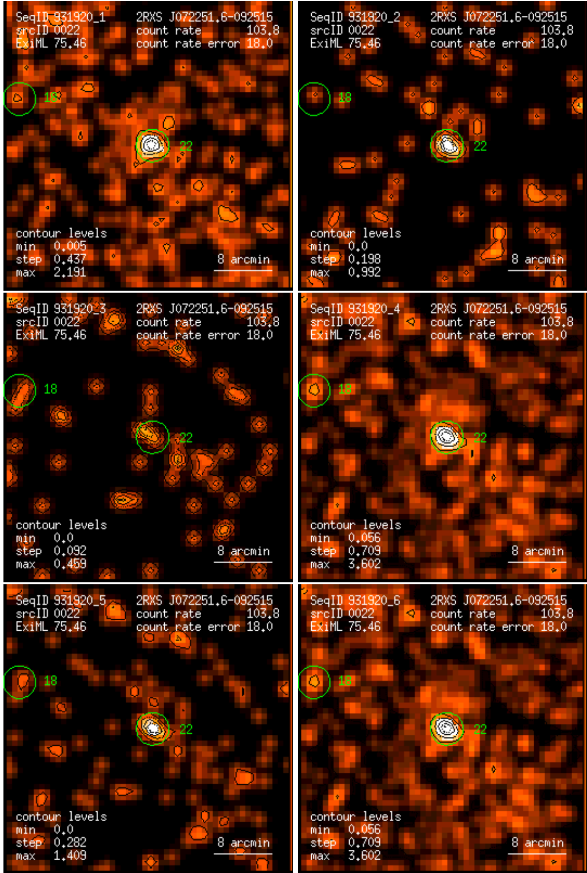
Figure 22: RASS 931920: detection 0022: band rate images, Gaussian filter: (1) PSPC channels 11 – 41, (2) 52 – 90, (3) 91 – 201, (4) 11 – 235, (5) 52 – 201, (6) 11 – 201. Broad band rates in counts/ks. Band rate contour levels in counts/ks/arcmin 2 .
