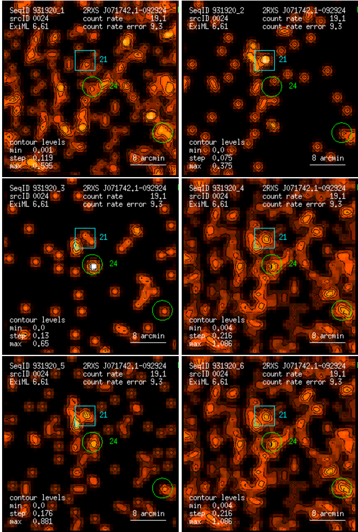
Figure 24: RASS 931920: detection 0024: band rate images, Gaussian filter: (1) PSPC channels 11 – 41, (2) 52 – 90, (3) 91 – 201, (4) 11 – 235, (5) 52 – 201, (6) 11 – 201. Broad band rates in counts/ks. Band rate contour levels in counts/ks/arcmin 2 .
