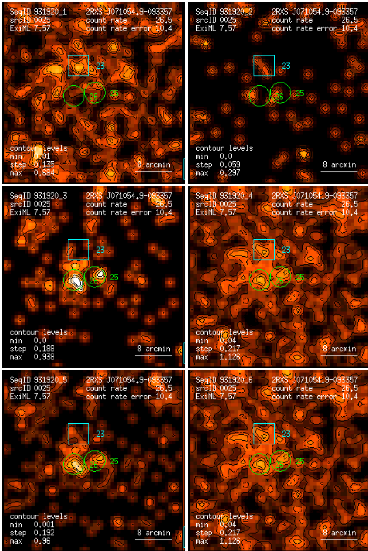
Figure 25: RASS 931920: detection 0025: band rate images, Gaussian filter: (1) PSPC channels 11 – 41, (2) 52 – 90, (3) 91 – 201, (4) 11 – 235, (5) 52 – 201, (6) 11 – 201. Broad band rates in counts/ks. Band rate contour levels in counts/ks/arcmin 2 .
