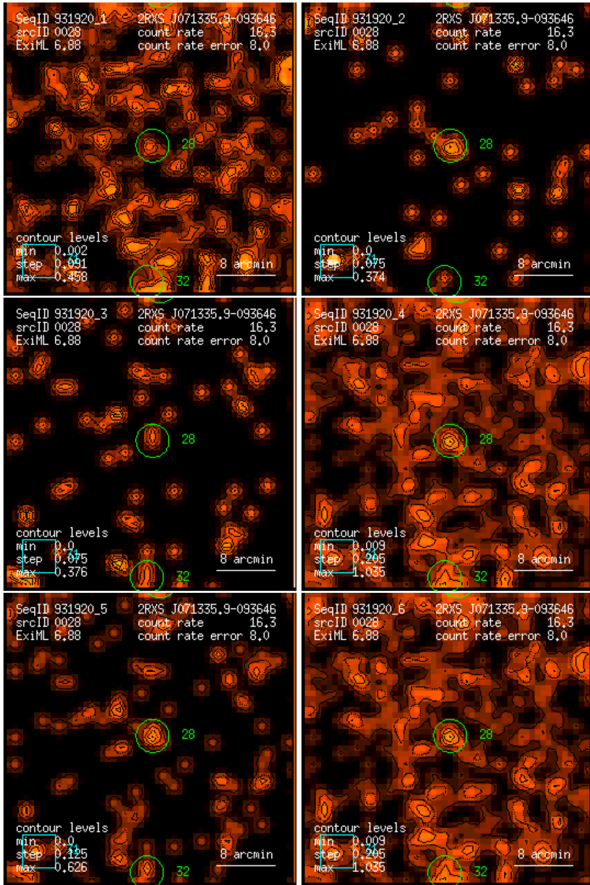
Figure 28: RASS 931920: detection 0028: band rate images, Gaussian filter: (1) PSPC channels 11 – 41, (2) 52 – 90, (3) 91 – 201, (4) 11 – 235, (5) 52 – 201, (6) 11 – 201. Broad band rates in counts/ks. Band rate contour levels in counts/ks/arcmin 2 .
