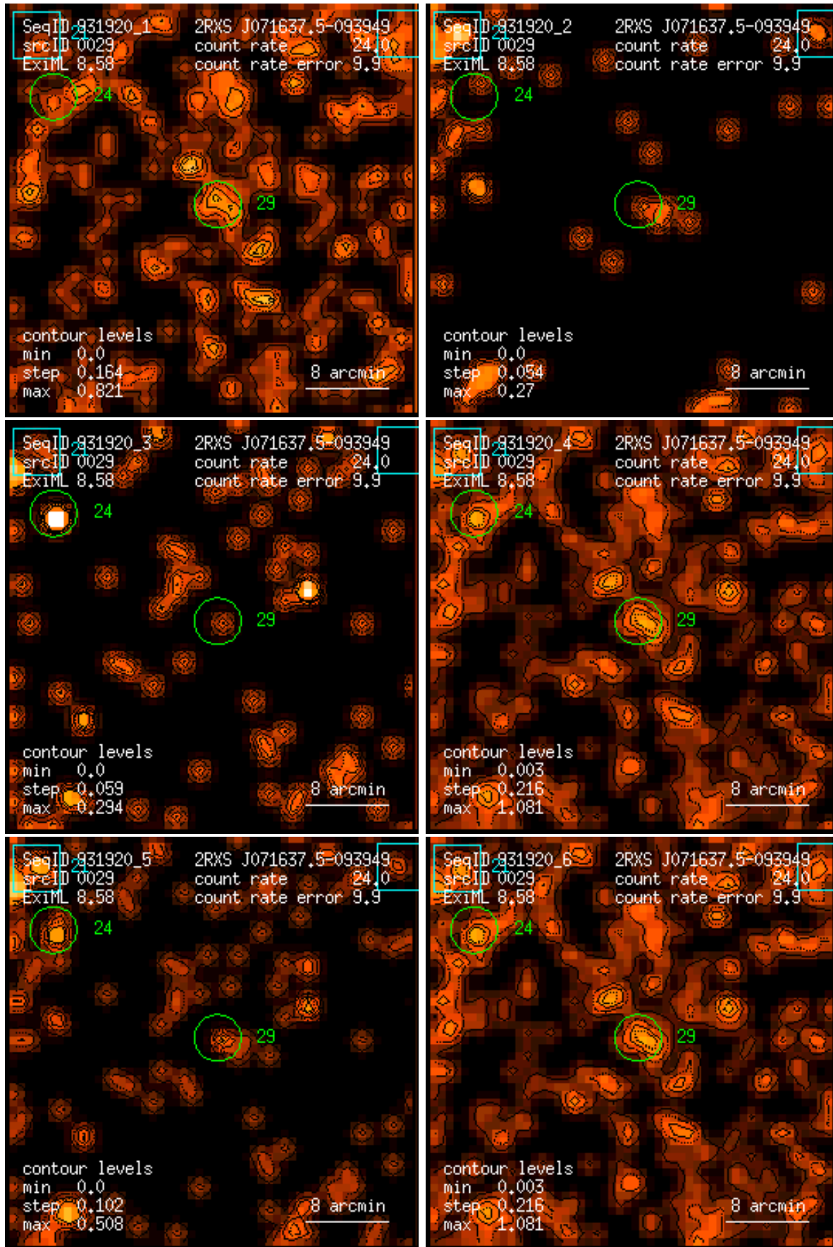
Figure 29: RASS 931920: detection 0029: band rate images, Gaussian filter: (1) PSPC channels 11 – 41, (2) 52 – 90, (3) 91 – 201, (4) 11 – 235, (5) 52 – 201, (6) 11 – 201. Broad band rates in counts/ks. Band rate contour levels in counts/ks/arcmin 2 .
