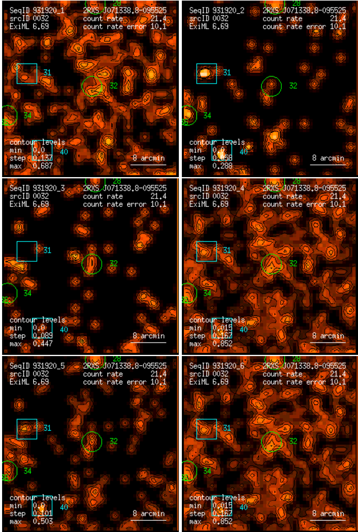
Figure 32: RASS 931920: detection 0032: band rate images, Gaussian filter: (1) PSPC channels 11 – 41, (2) 52 – 90, (3) 91 – 201, (4) 11 – 235, (5) 52 – 201, (6) 11 – 201. Broad band rates in counts/ks. Band rate contour levels in counts/ks/arcmin 2 .
