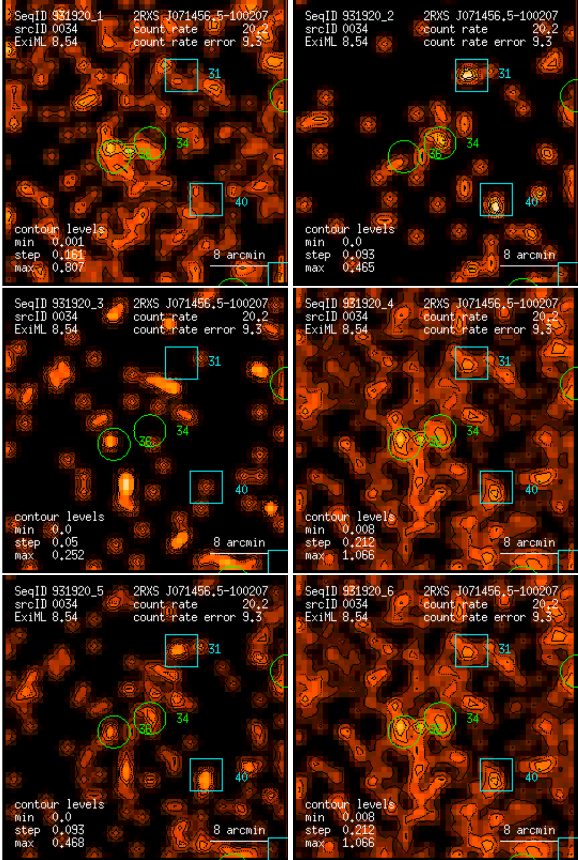
Figure 34: RASS 931920: detection 0034: band rate images, Gaussian filter: (1) PSPC channels 11 – 41, (2) 52 – 90, (3) 91 – 201, (4) 11 – 235, (5) 52 – 201, (6) 11 – 201. Broad band rates in counts/ks. Band rate contour levels in counts/ks/arcmin 2 .
