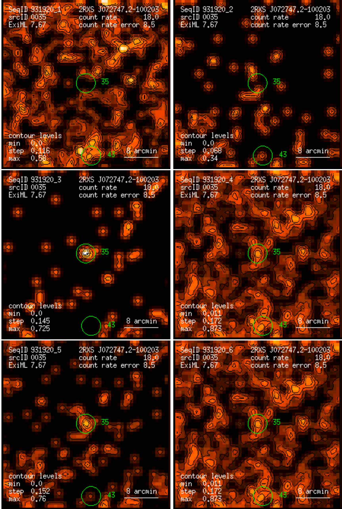
Figure 35: RASS 931920: detection 0035: band rate images, Gaussian filter: (1) PSPC channels 11 – 41, (2) 52 – 90, (3) 91 – 201, (4) 11 – 235, (5) 52 – 201, (6) 11 – 201. Broad band rates in counts/ks. Band rate contour levels in counts/ks/arcmin 2 .
