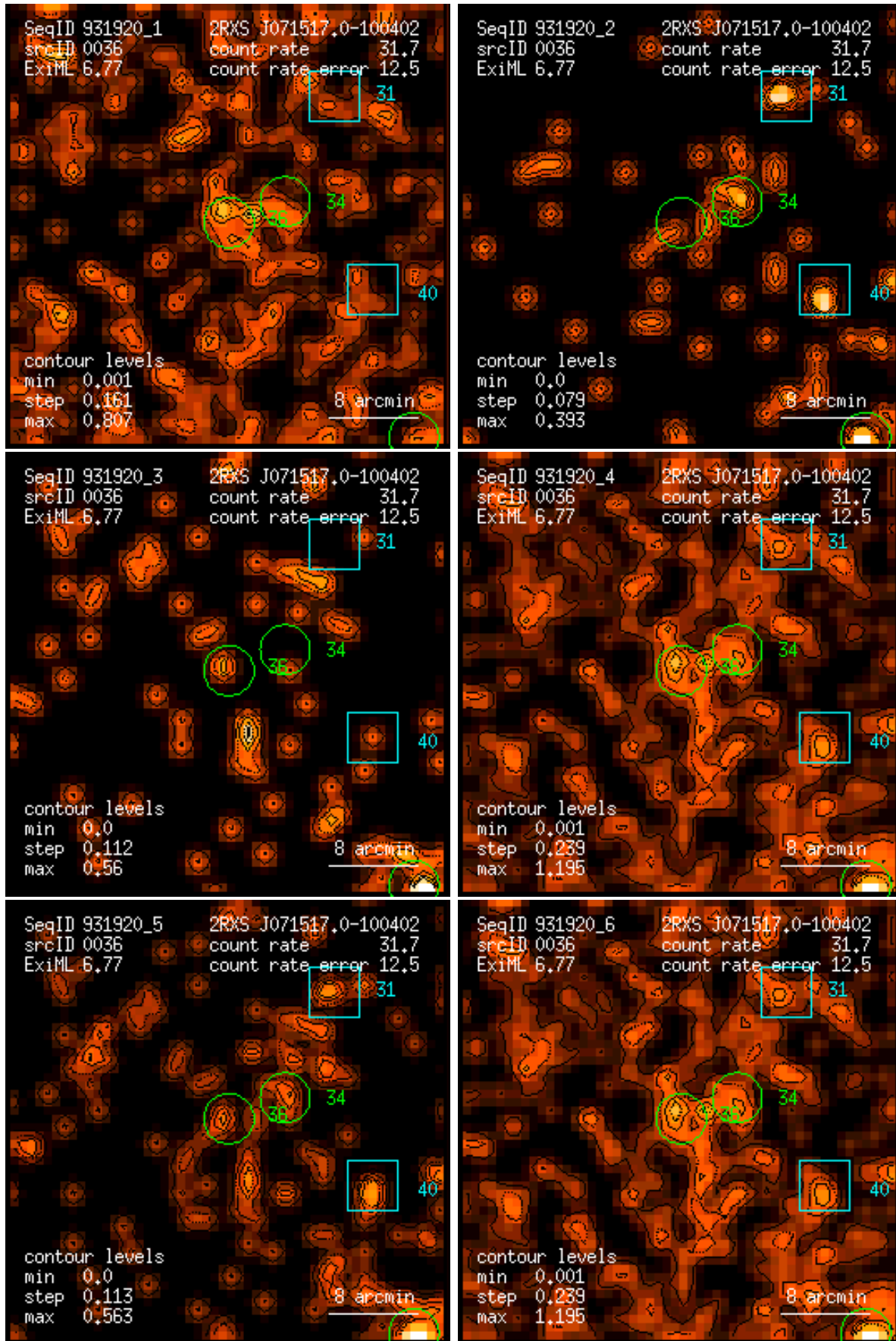
Figure 36: RASS 931920: detection 0036: band rate images, Gaussian filter: (1) PSPC channels 11 – 41, (2) 52 – 90, (3) 91 – 201, (4) 11 – 235, (5) 52 – 201, (6) 11 – 201. Broad band rates in counts/ks. Band rate contour levels in counts/ks/arcmin 2 .
