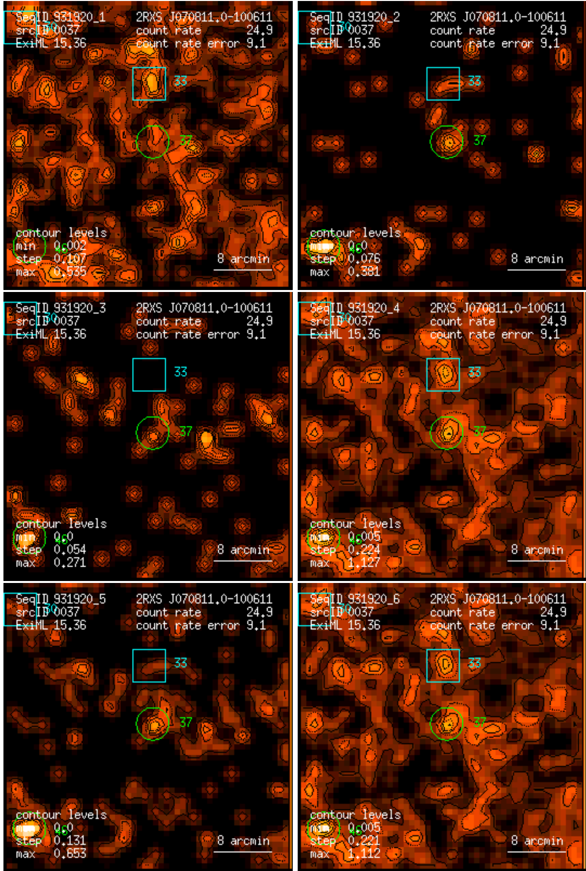
Figure 37: RASS 931920: detection 0037: band rate images, Gaussian filter: (1) PSPC channels 11 – 41, (2) 52 – 90, (3) 91 – 201, (4) 11 – 235, (5) 52 – 201, (6) 11 – 201. Broad band rates in counts/ks. Band rate contour levels in counts/ks/arcmin 2 .
