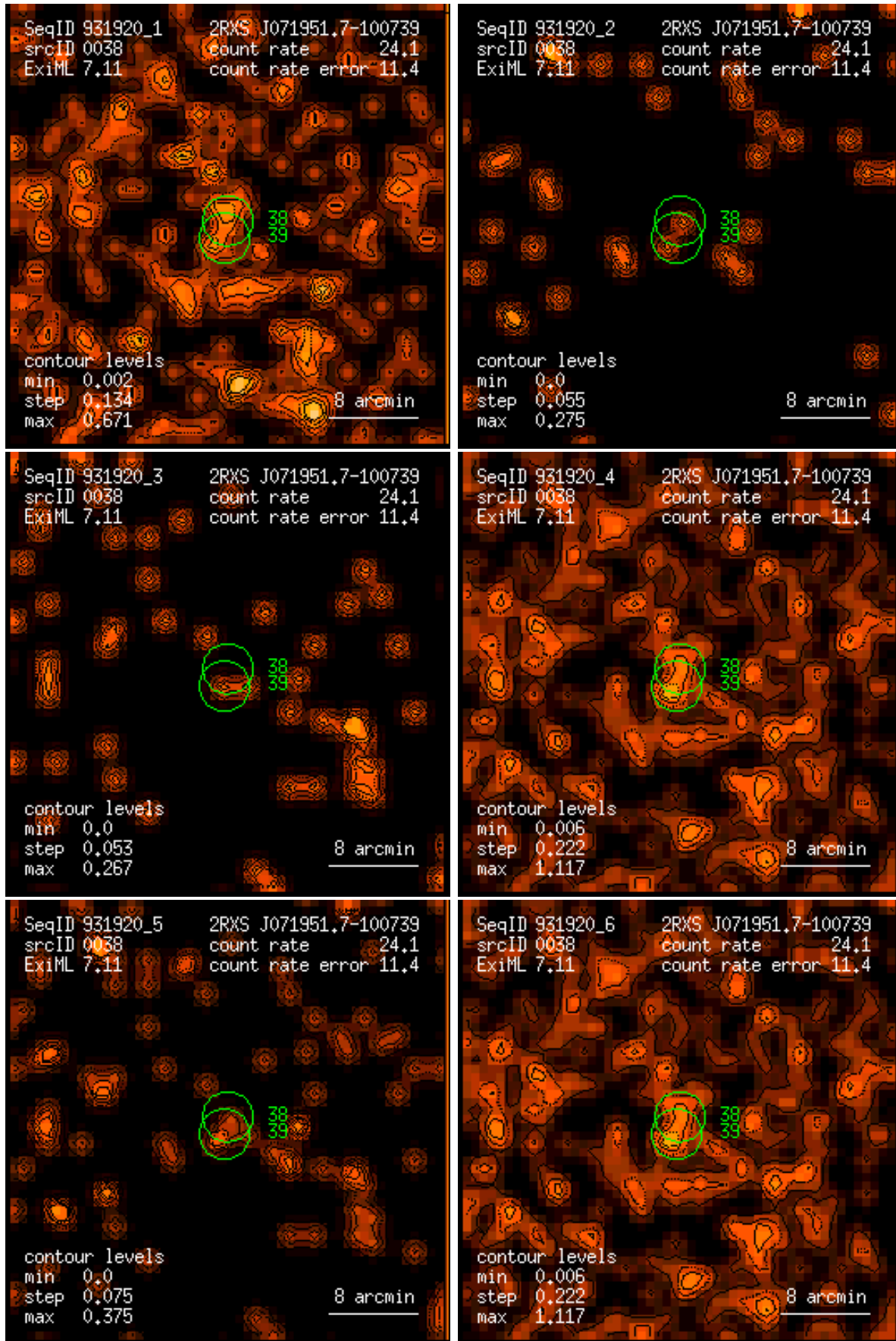
Figure 38: RASS 931920: detection 0038: band rate images, Gaussian filter: (1) PSPC channels 11 – 41, (2) 52 – 90, (3) 91 – 201, (4) 11 – 235, (5) 52 – 201, (6) 11 – 201. Broad band rates in counts/ks. Band rate contour levels in counts/ks/arcmin 2 .
