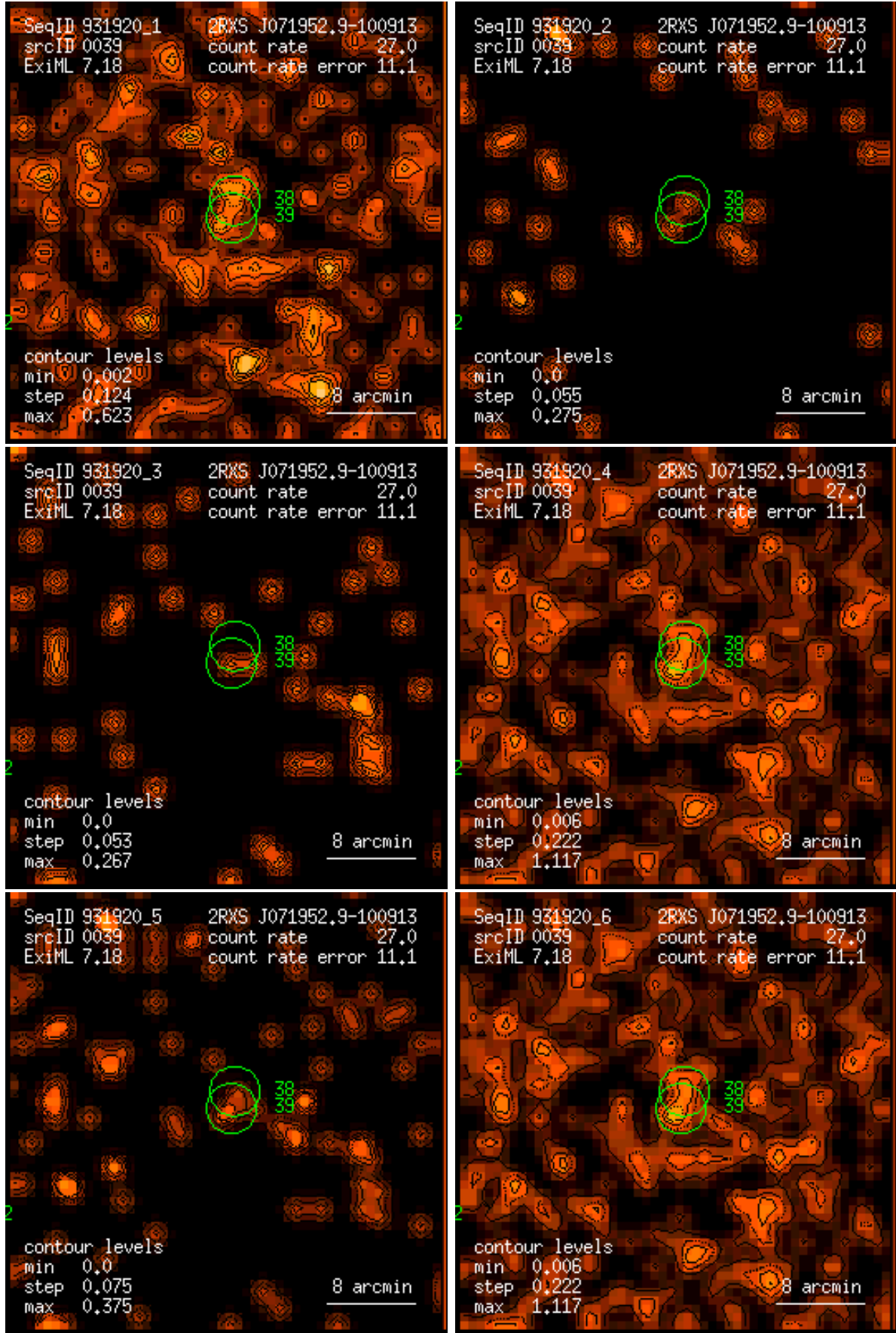
Figure 39: RASS 931920: detection 0039: band rate images, Gaussian filter: (1) PSPC channels 11 – 41, (2) 52 – 90, (3) 91 – 201, (4) 11 – 235, (5) 52 – 201, (6) 11 – 201. Broad band rates in counts/ks. Band rate contour levels in counts/ks/arcmin 2 .
