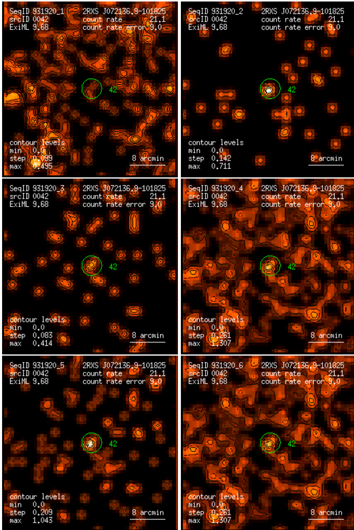
Figure 42: RASS 931920: detection 0042: band rate images, Gaussian filter: (1) PSPC channels 11 – 41, (2) 52 – 90, (3) 91 – 201, (4) 11 – 235, (5) 52 – 201, (6) 11 – 201. Broad band rates in counts/ks. Band rate contour levels in counts/ks/arcmin 2 .
