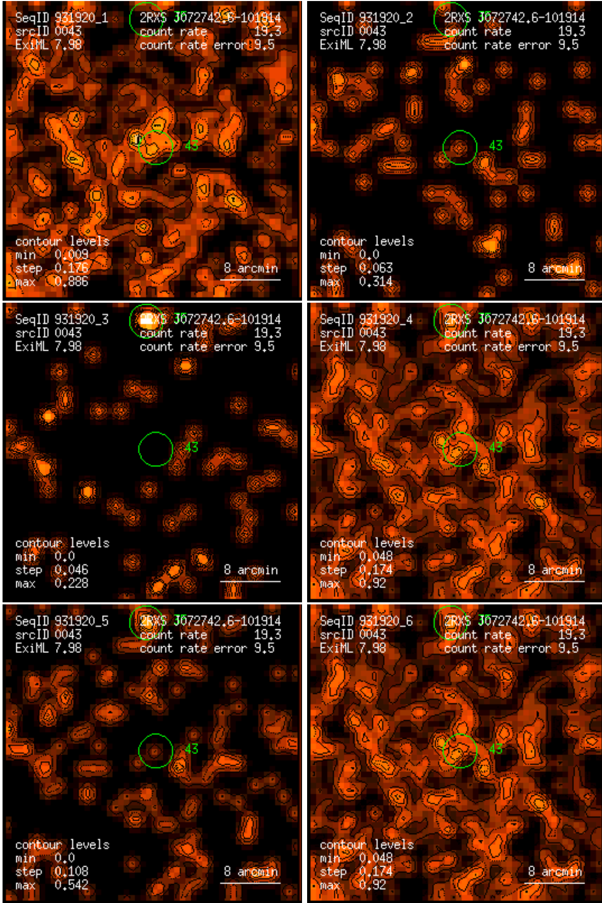
Figure 43: RASS 931920: detection 0043: band rate images, Gaussian filter: (1) PSPC channels 11 – 41, (2) 52 – 90, (3) 91 – 201, (4) 11 – 235, (5) 52 – 201, (6) 11 – 201. Broad band rates in counts/ks. Band rate contour levels in counts/ks/arcmin 2 .
