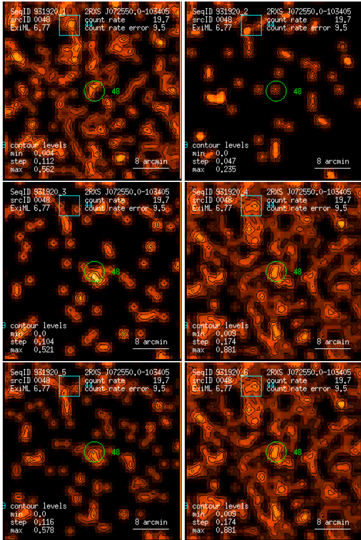
Figure 48: RASS 931920: detection 0048: band rate images, Gaussian filter: (1) PSPC channels 11 – 41, (2) 52 – 90, (3) 91 – 201, (4) 11 – 235, (5) 52 – 201, (6) 11 – 201. Broad band rates in counts/ks. Band rate contour levels in counts/ks/arcmin 2 .
