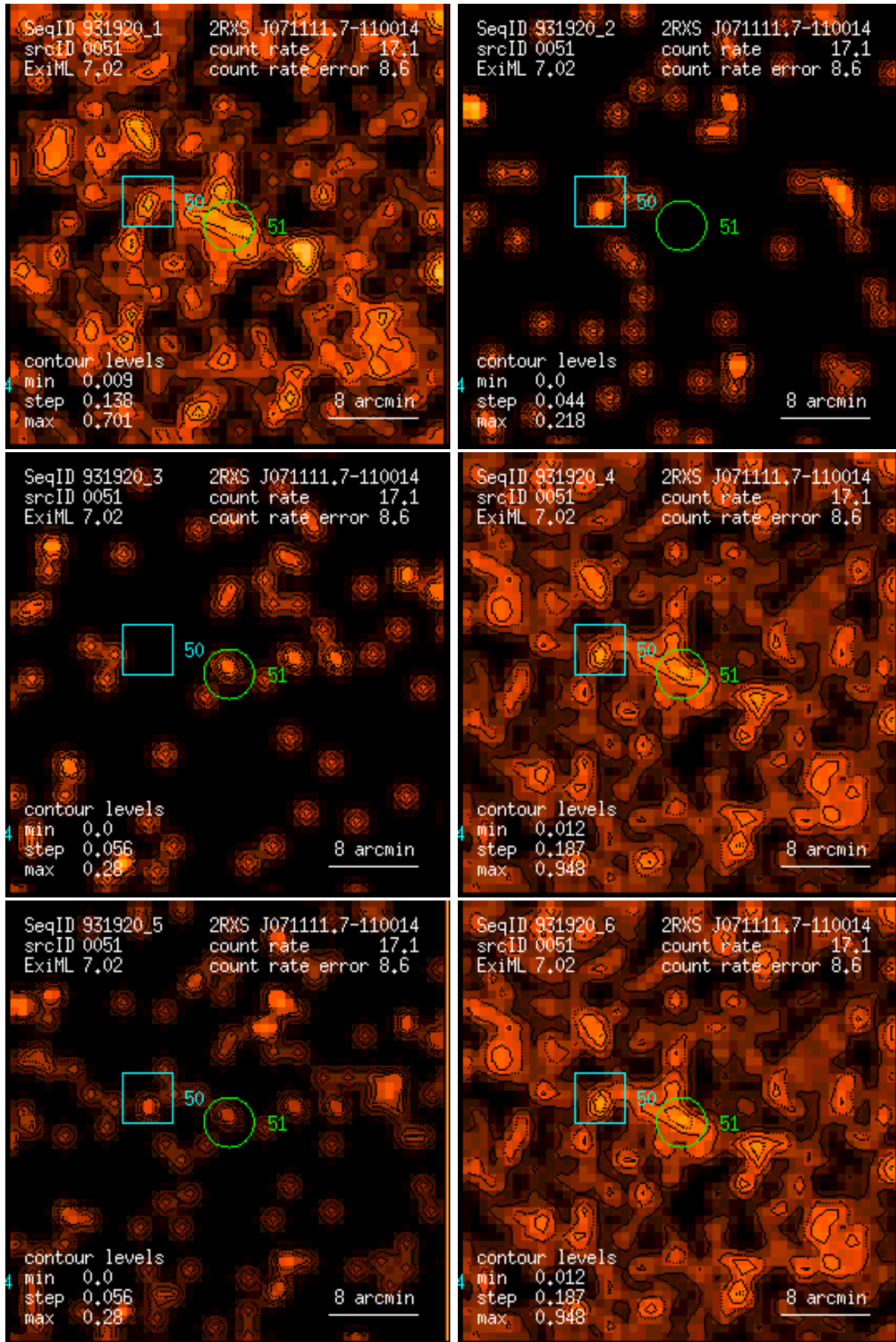
Figure 51: RASS 931920: detection 0051: band rate images, Gaussian filter: (1) PSPC channels 11 – 41, (2) 52 – 90, (3) 91 – 201, (4) 11 – 235, (5) 52 – 201, (6) 11 – 201. Broad band rates in counts/ks. Band rate contour levels in counts/ks/arcmin 2 .
