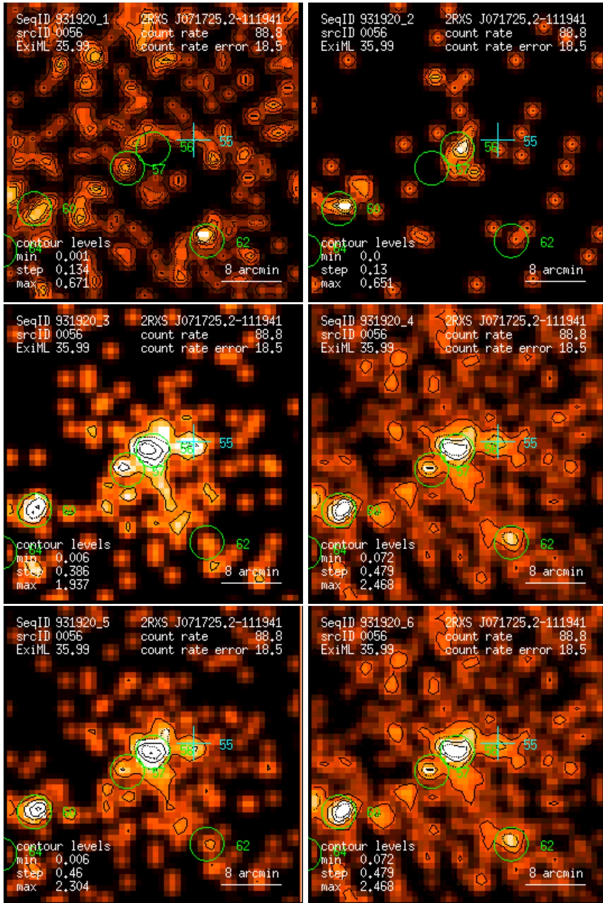
Figure 56: RASS 931920: detection 0056: band rate images, Gaussian filter: (1) PSPC channels 11 – 41, (2) 52 – 90, (3) 91 – 201, (4) 11 – 235, (5) 52 – 201, (6) 11 – 201. Broad band rates in counts/ks. Band rate contour levels in counts/ks/arcmin 2 .
