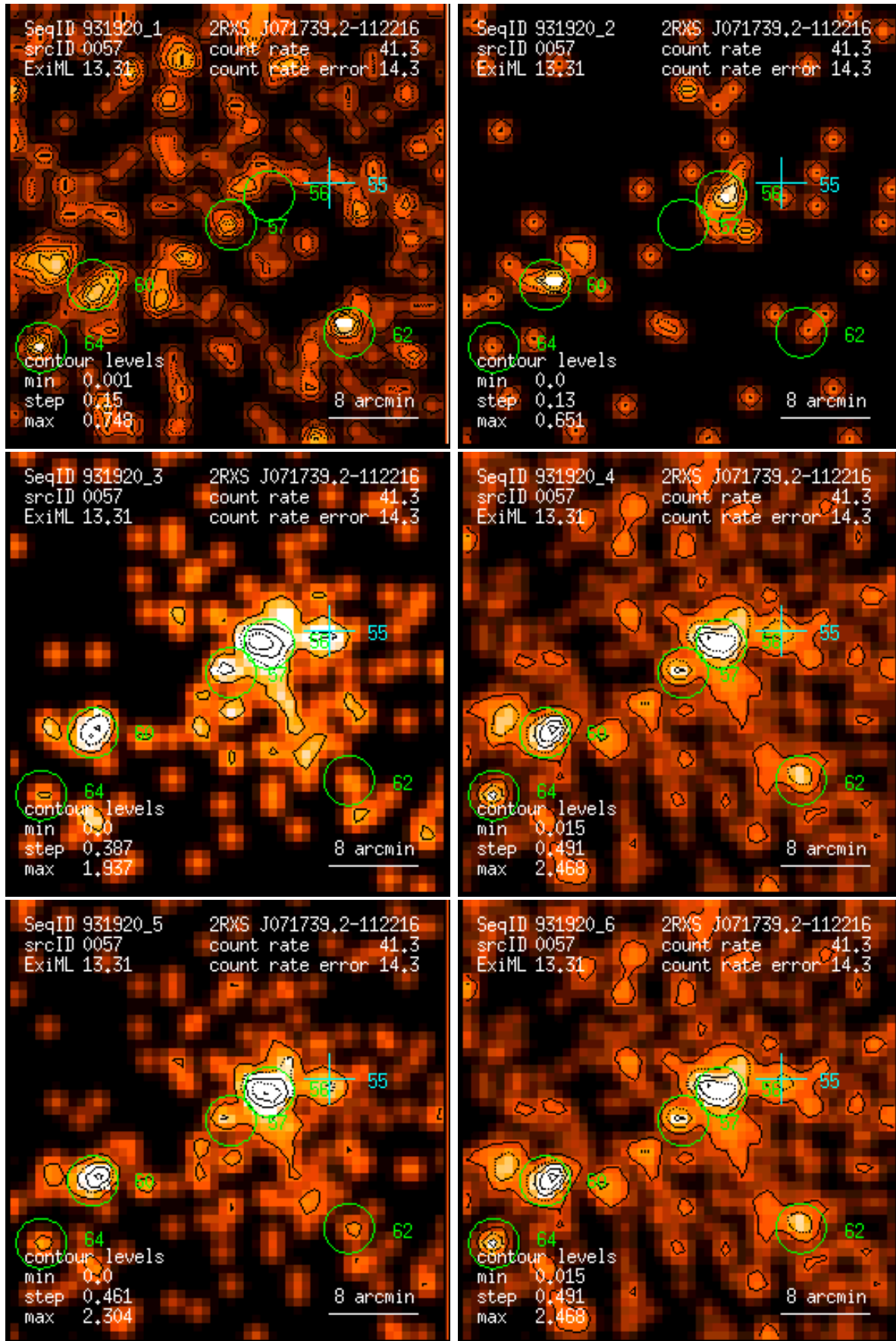
Figure 57: RASS 931920: detection 0057: band rate images, Gaussian filter: (1) PSPC channels 11 – 41, (2) 52 – 90, (3) 91 – 201, (4) 11 – 235, (5) 52 – 201, (6) 11 – 201. Broad band rates in counts/ks. Band rate contour levels in counts/ks/arcmin 2 .
