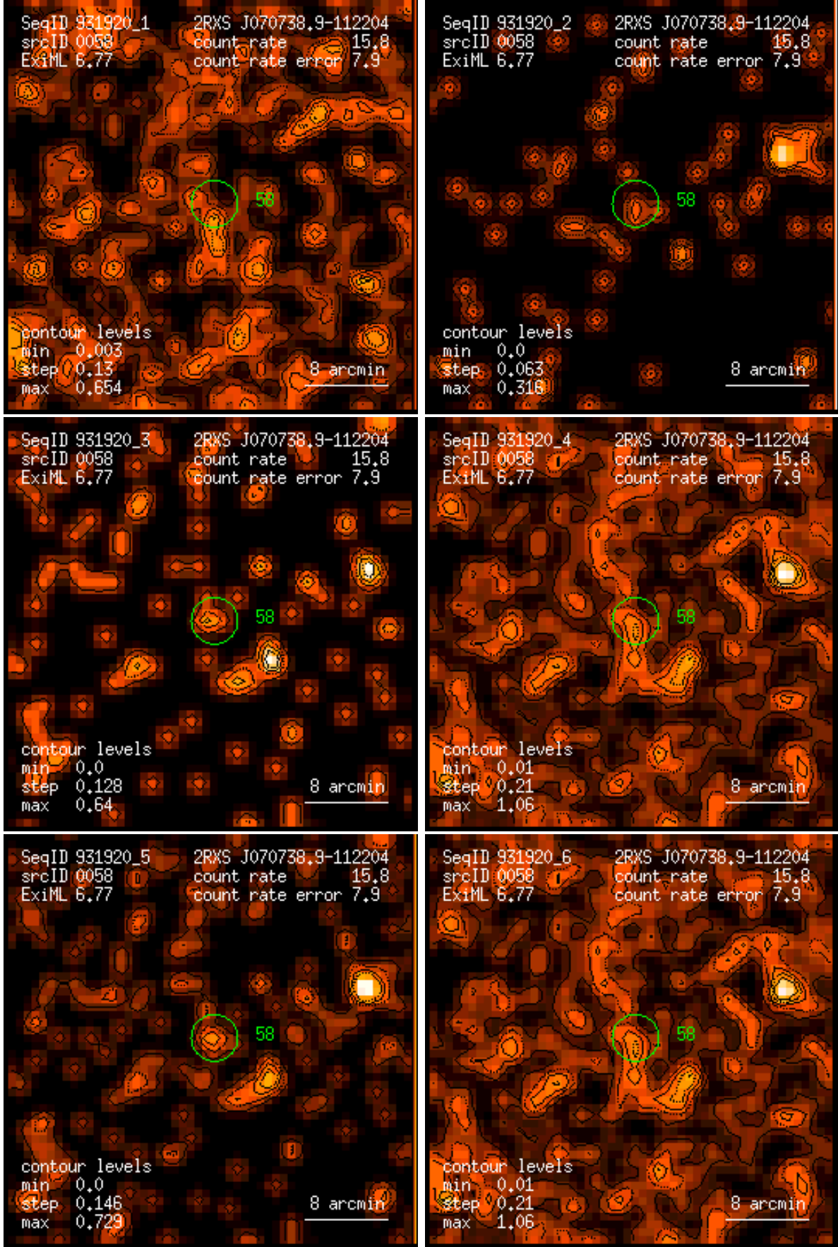
Figure 58: RASS 931920: detection 0058: band rate images, Gaussian filter: (1) PSPC channels 11 – 41, (2) 52 – 90, (3) 91 – 201, (4) 11 – 235, (5) 52 – 201, (6) 11 – 201. Broad band rates in counts/ks. Band rate contour levels in counts/ks/arcmin 2 .
