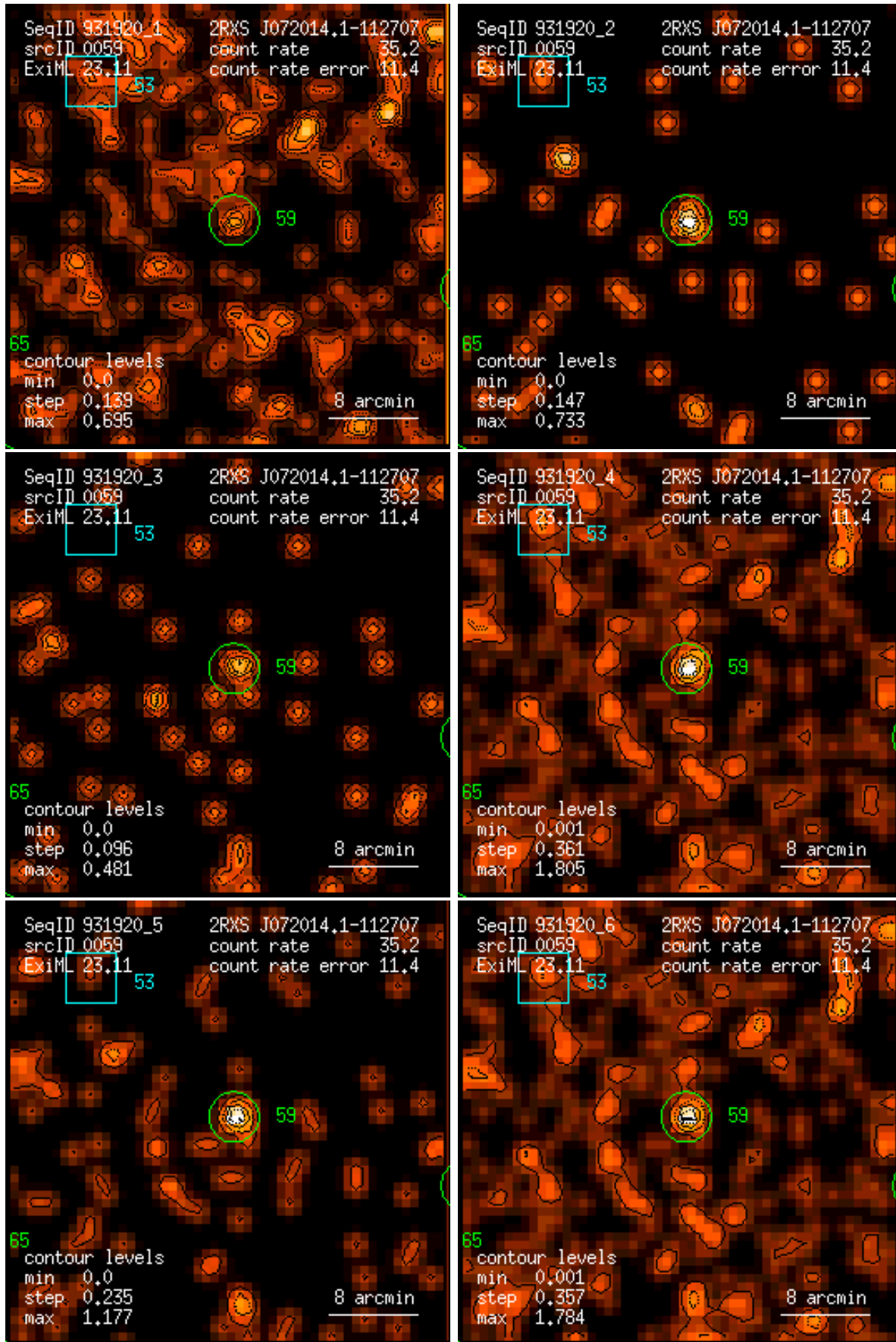
Figure 59: RASS 931920: detection 0059: band rate images, Gaussian filter: (1) PSPC channels 11 – 41, (2) 52 – 90, (3) 91 – 201, (4) 11 – 235, (5) 52 – 201, (6) 11 – 201. Broad band rates in counts/ks. Band rate contour levels in counts/ks/arcmin 2 .
