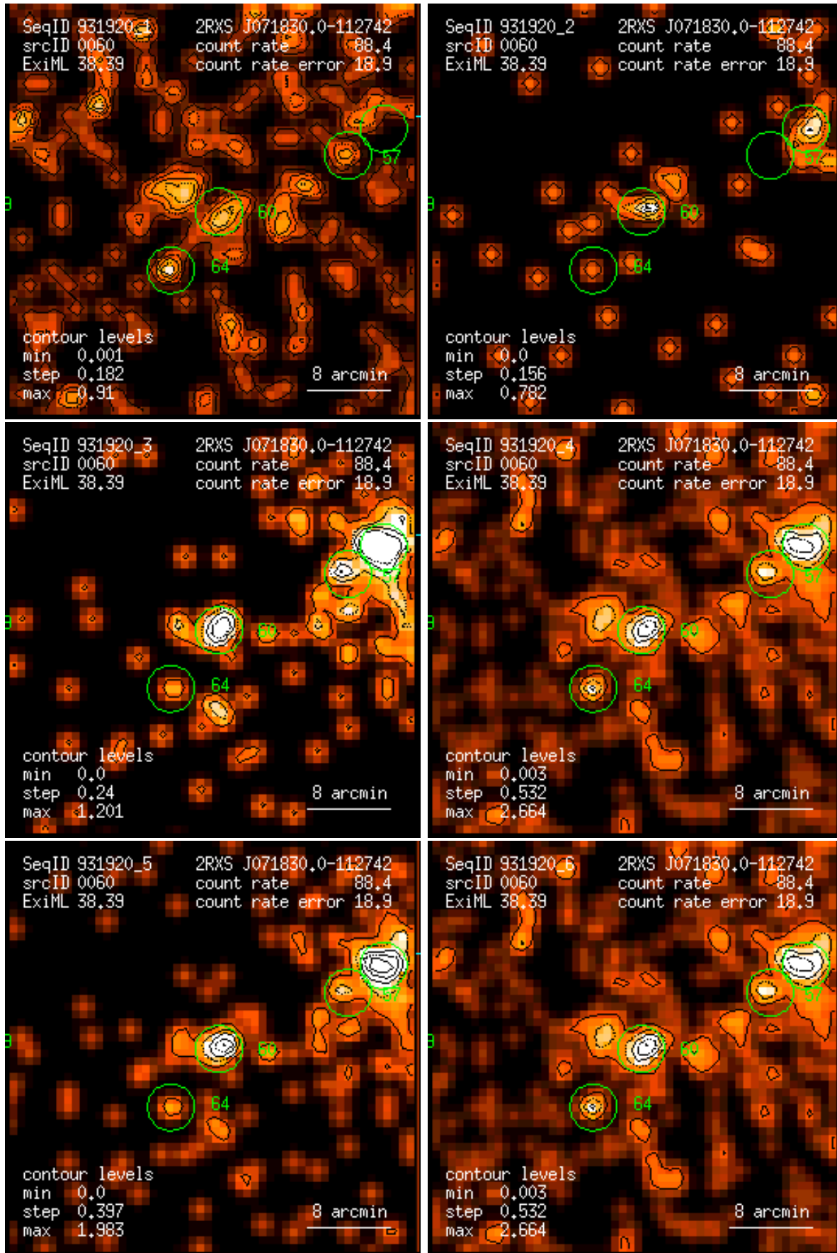
Figure 60: RASS 931920: detection 0060: band rate images, Gaussian filter: (1) PSPC channels 11 – 41, (2) 52 – 90, (3) 91 – 201, (4) 11 – 235, (5) 52 – 201, (6) 11 – 201. Broad band rates in counts/ks. Band rate contour levels in counts/ks/arcmin 2 .
