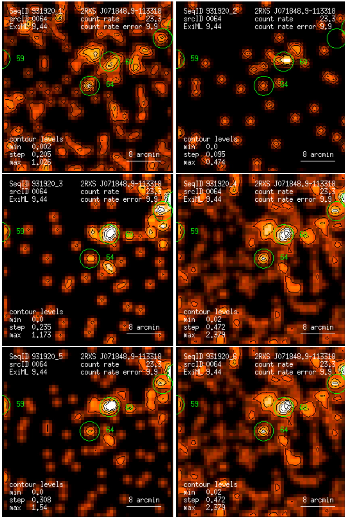
Figure 64: RASS 931920: detection 0064: band rate images, Gaussian filter: (1) PSPC channels 11 – 41, (2) 52 – 90, (3) 91 – 201, (4) 11 – 235, (5) 52 – 201, (6) 11 – 201. Broad band rates in counts/ks. Band rate contour levels in counts/ks/arcmin 2 .
