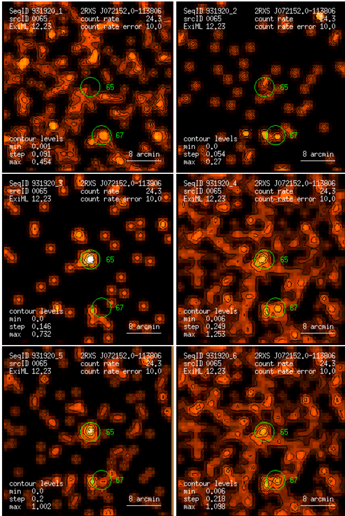
Figure 65: RASS 931920: detection 0065: band rate images, Gaussian filter: (1) PSPC channels 11 – 41, (2) 52 – 90, (3) 91 – 201, (4) 11 – 235, (5) 52 – 201, (6) 11 – 201. Broad band rates in counts/ks. Band rate contour levels in counts/ks/arcmin 2 .
