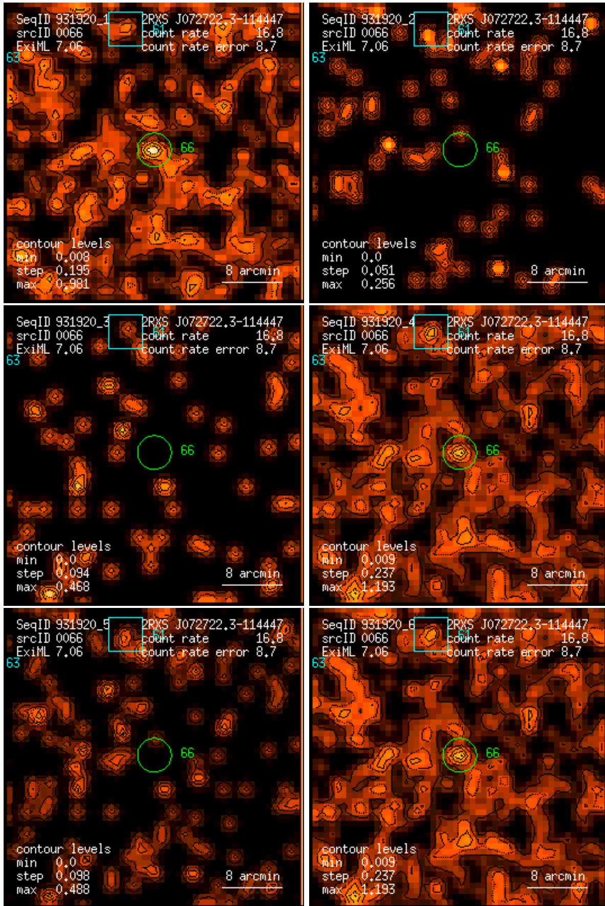
Figure 66: RASS 931920: detection 0066: band rate images, Gaussian filter: (1) PSPC channels 11 – 41, (2) 52 – 90, (3) 91 – 201, (4) 11 – 235, (5) 52 – 201, (6) 11 – 201. Broad band rates in counts/ks. Band rate contour levels in counts/ks/arcmin 2 .
