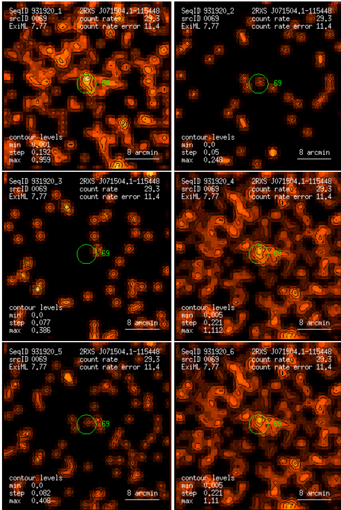
Figure 69: RASS 931920: detection 0069: band rate images, Gaussian filter: (1) PSPC channels 11 – 41, (2) 52 – 90, (3) 91 – 201, (4) 11 – 235, (5) 52 – 201, (6) 11 – 201. Broad band rates in counts/ks. Band rate contour levels in counts/ks/arcmin 2 .
