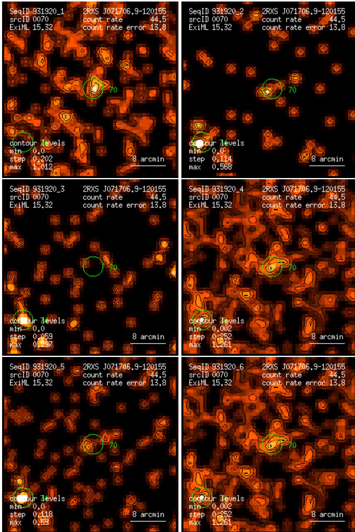
Figure 70: RASS 931920: detection 0070: band rate images, Gaussian filter: (1) PSPC channels 11 – 41, (2) 52 – 90, (3) 91 – 201, (4) 11 – 235, (5) 52 – 201, (6) 11 – 201. Broad band rates in counts/ks. Band rate contour levels in counts/ks/arcmin 2 .
